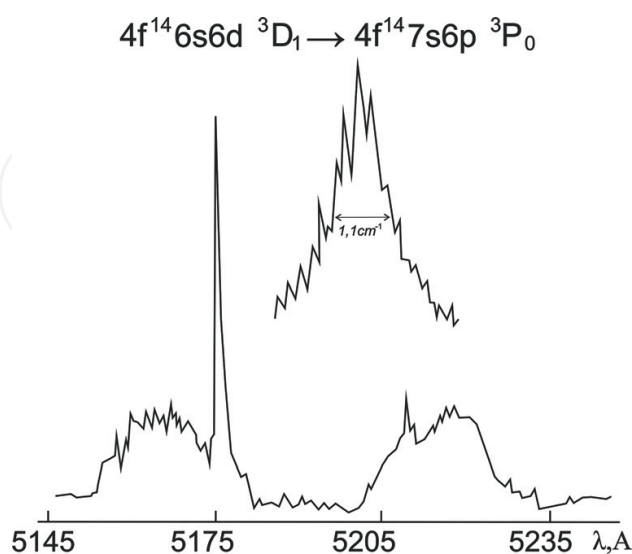
Figure 2. Dependence of ion current on the third stage laser wavelength, under excitation of the AS 7s6p \text{ } ^3P_0^0 from the 6s6d^3D_1 state by laser radiation with the line width of \sim 1 \text{ cm}^{-1} .
