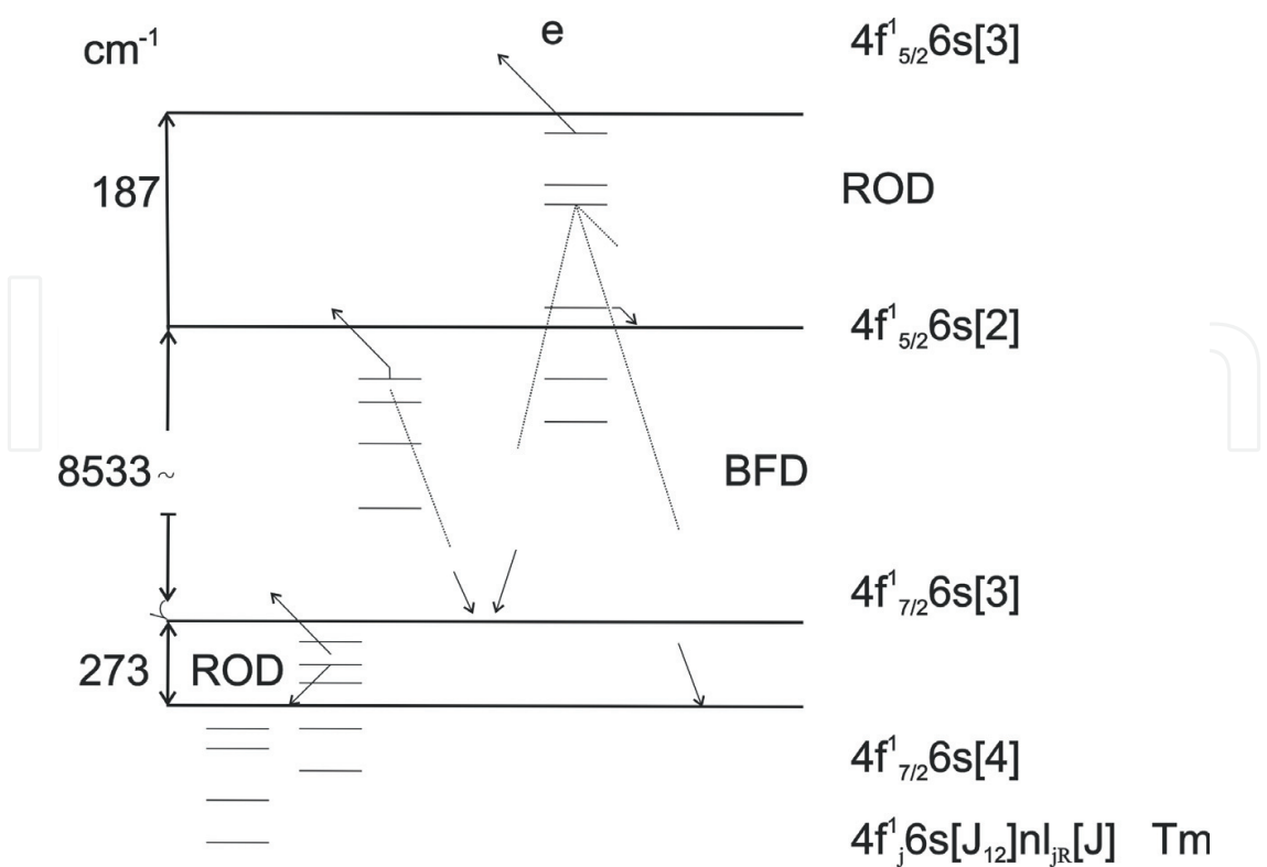
Figure 3. Position of the low-lying Tm atom 4f 1 6snl ionization limits and scheme of autoionization decay of Tm atom Rydberg states 4f 13 6snl.
