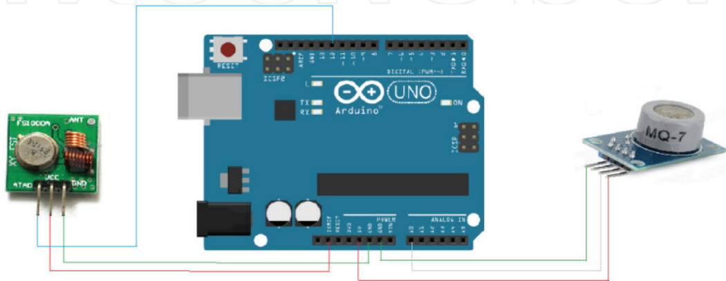
Figure 8. Transmitter setup.
