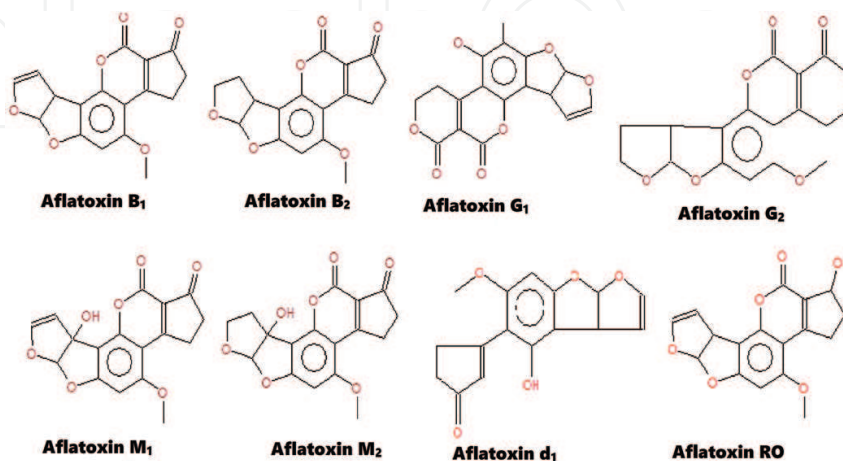
Figure 1. Structure of aflatoxins.
