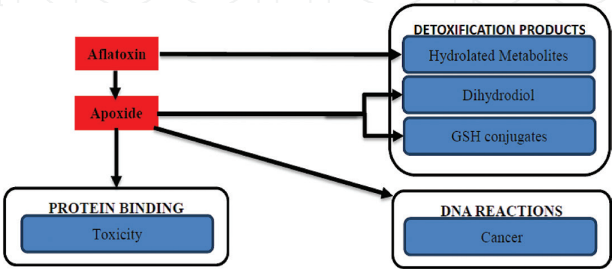
Figure 2. Aflatoxin metabolism in humans.
