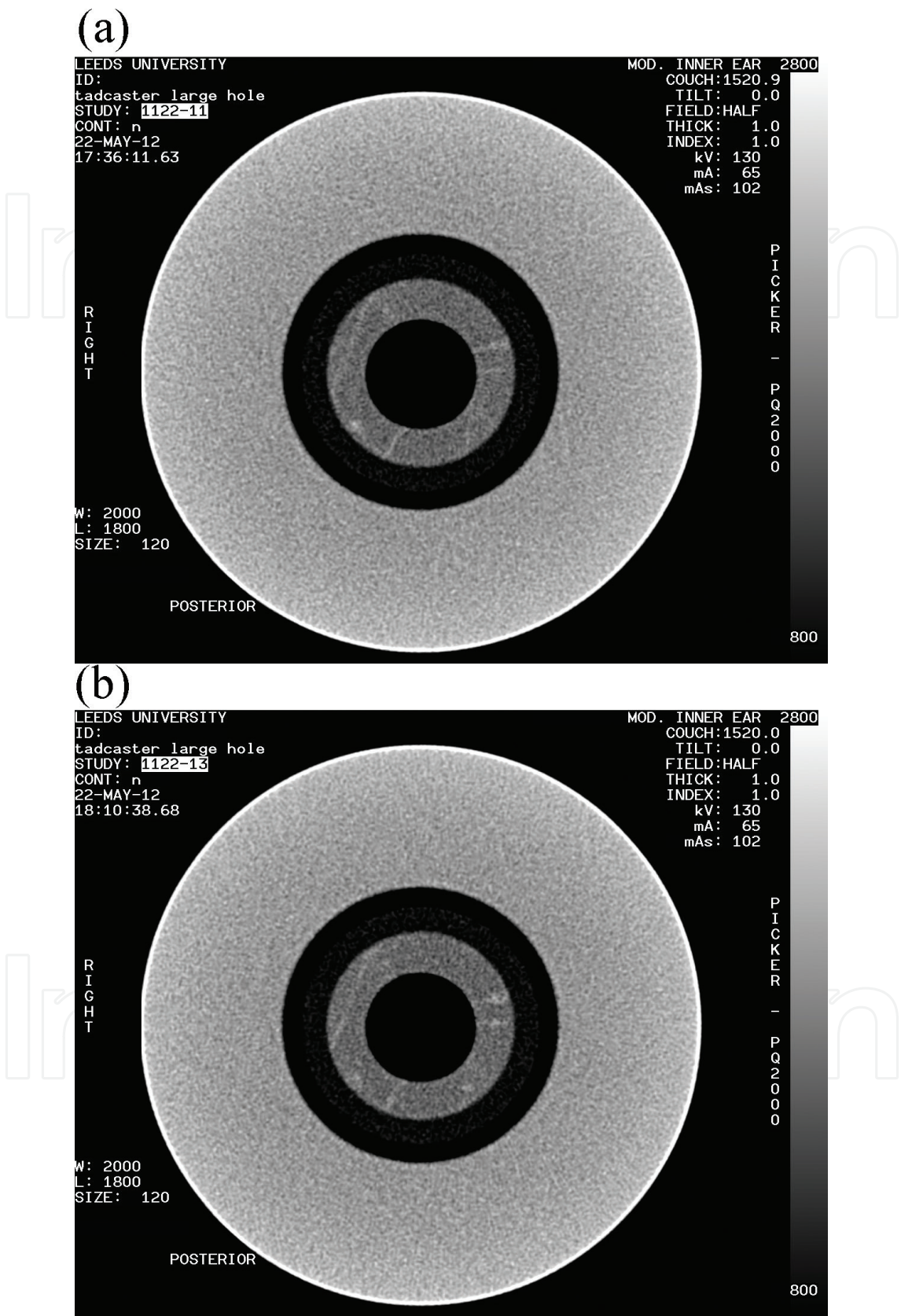
Figure 23. Scan images of the large cavity limestone specimen at different times before the initiation of fractures. (a) Early stage, (b) Later stage.
