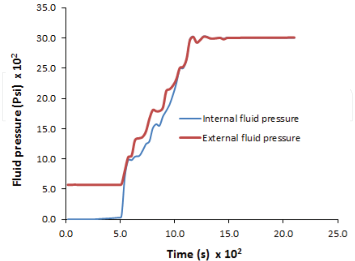
Figure 13. External and internal fluid pressure during injection (strongest sample).
