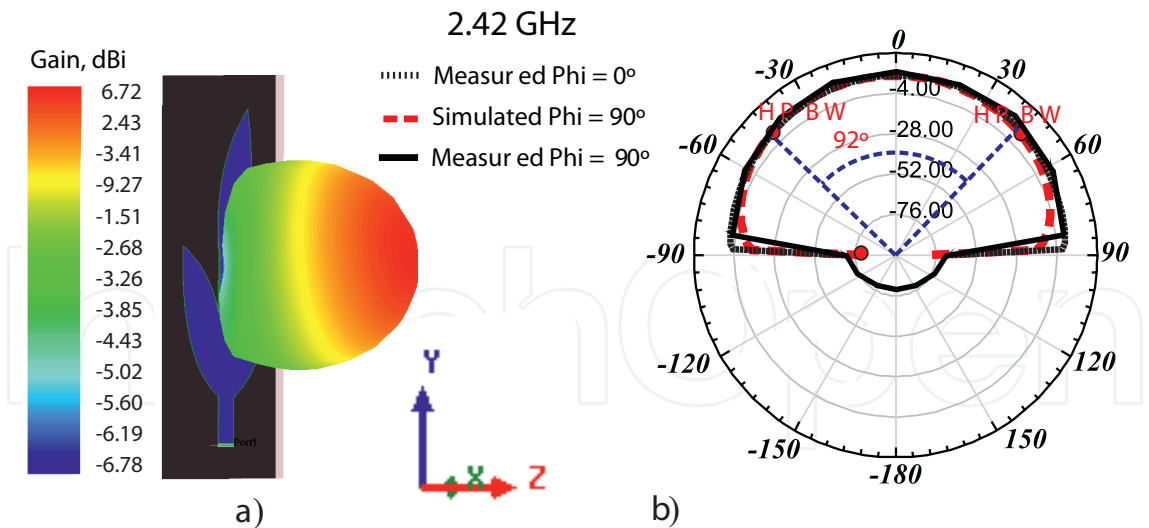
Figure 23. Radiation pattern of the bio-inspired textile antenna: (a) 3D with antenna structure, (b) 2D with HPBW and relative F/B.
