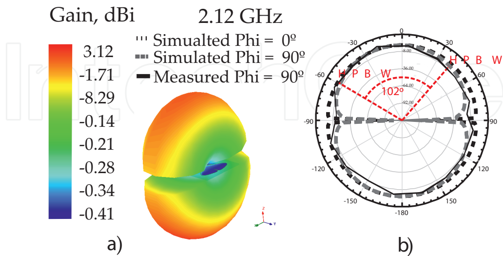
Figure 19. 2D and 3D radiation pattern of the antenna proposed.
