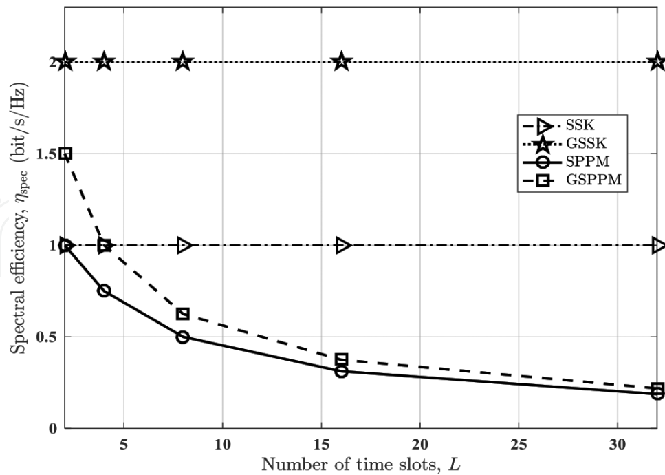
Figure 11. Spectral efficiency comparison of optical SM schemes.
