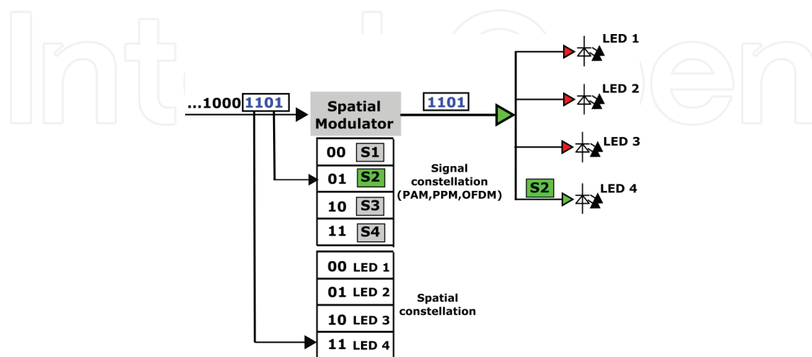
Figure 1. An illustration of the encoding mechanism of an optical SM technique.
