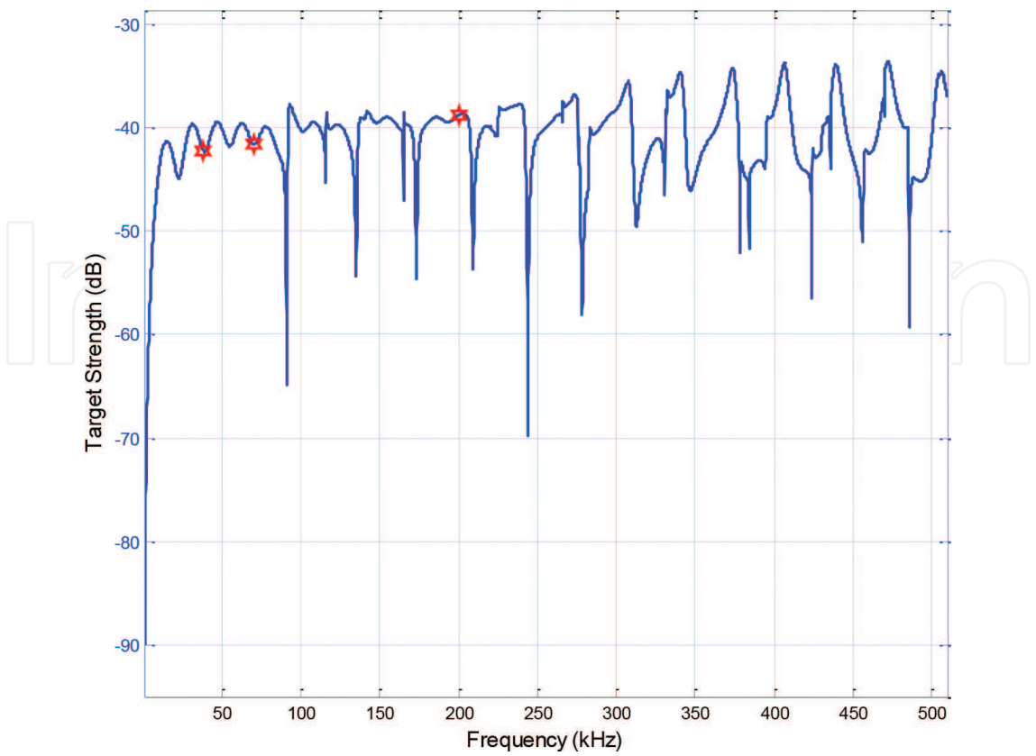
Figure 4. Measurement (*) and theoretical target strength (-).
