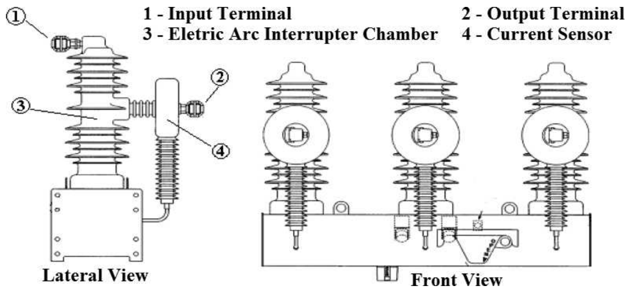
Figure 2. Recloser.
