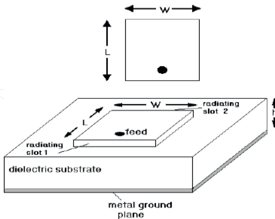
Figure 1. Basic layout of rectangular patch antenna.
