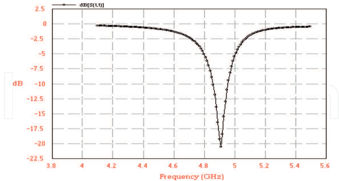
Figure 7. Simulated response of patch at 4.89 GHz resonant frequency.
