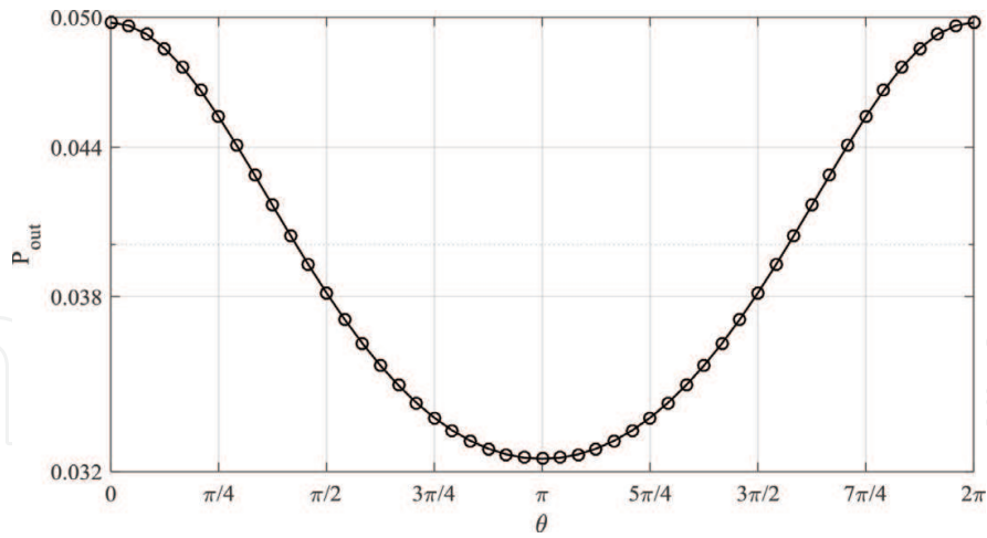
Figure 2. P_{out} for the considered underlay CR network with DF relaying under different \theta values.
