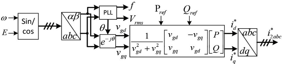
Figure 12. Generation of reference current i_{2abc}^* after islanding occurs.
