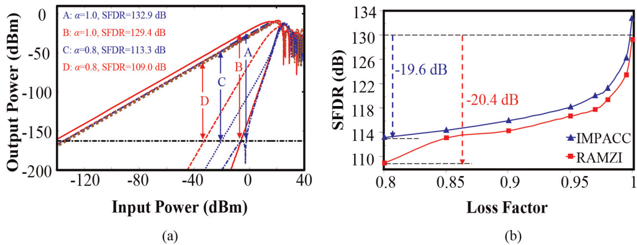
Figure 13. (a) Effect of MRR waveguide loss, \alpha on the SFDRs of IMPACC and RAMZI for \omega_m = 1\text{ Hz} ( F , \xi_{PM} are fixed), (A) IMPACC with \alpha = 1 , (B) RAMZI with \alpha = 1 , (C) IMPACC with \alpha = 0.8 , (D) RAMZI with \alpha = 0.8 ; (b) effect of different values of MRR loss factor on the SFDR values for IMPACC and RAMZI.
