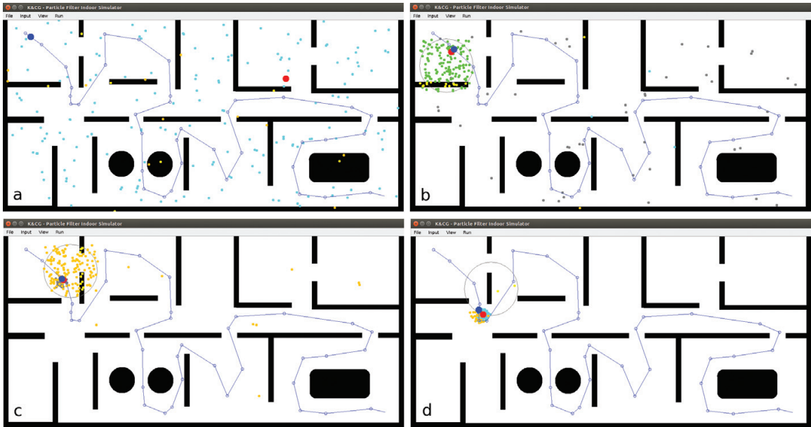
Figure 4. Particle filter in action: 100 particles were randomly located in the building (a), a WiFi positioning service was used for fast converges (b and c). All the particles converged to the correct position (d).
