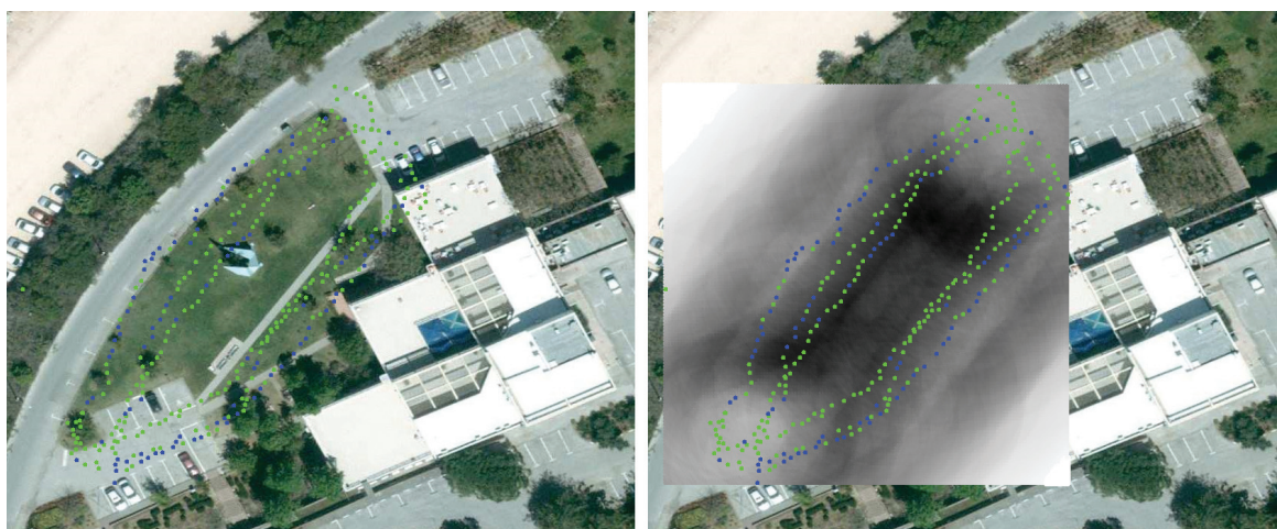
Figure 8. A heat map algorithm: No active jammer. Left: All samples. Right: The brightest regions of heat map are at the upper left and lower right corners. Since no jammer exists, the algorithm assumes it is outside the ROI.
