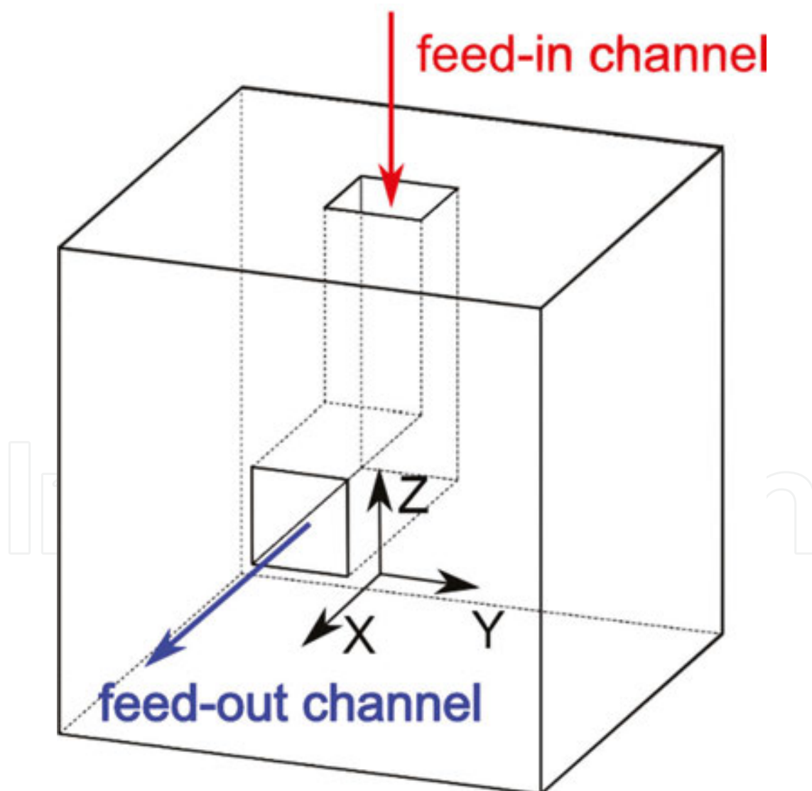
Figure 1. The scheme of the ECAP die including the coordinate system [2].
