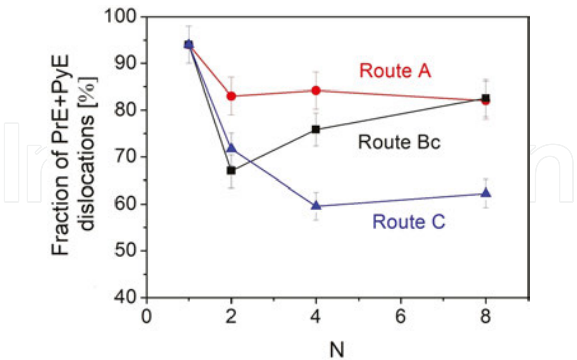
Figure 19. The dependence of the sum of relative fractions of prismatic (PrE) and pyramidal (PyE) \langle a \rangle -type edge dislocations on the route of ECAP and the number of passes.
