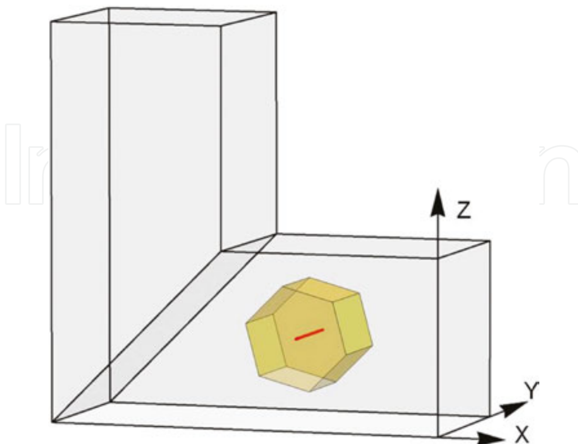
Figure 27. The formation mechanism of the texture component L.
