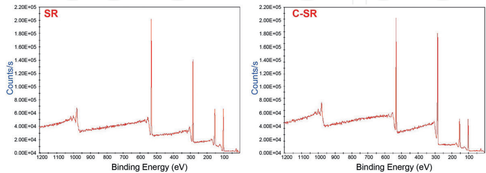
Figure 6. XPS results of virgin silicone rubber and carbon ion-implanted silicone rubber.
