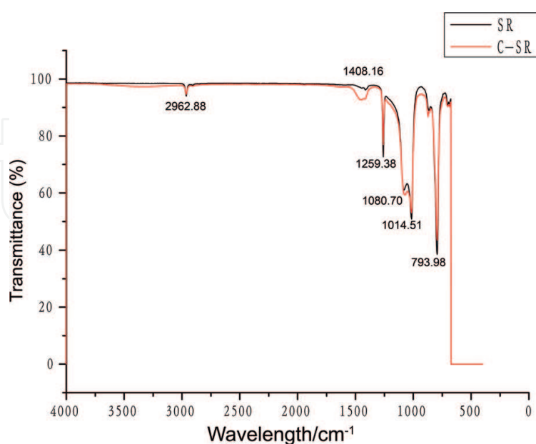
Figure 2. The Fourier transformation infrared spectroscopy results of virgin silicone rubber and carbon ion-implanted silicone rubber.
