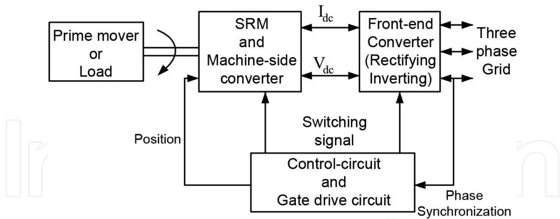
Figure 2. A block diagram of a two-stage converter.
