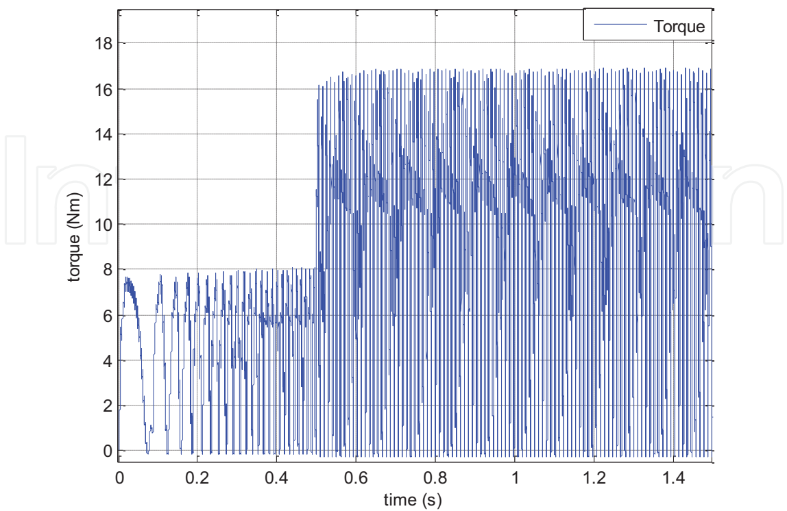
Figure 18. SRM torque.
