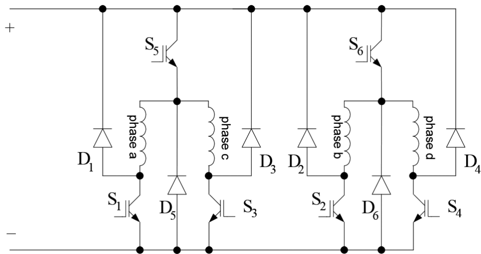
Figure 3. 1.5 switch/phase converter.
