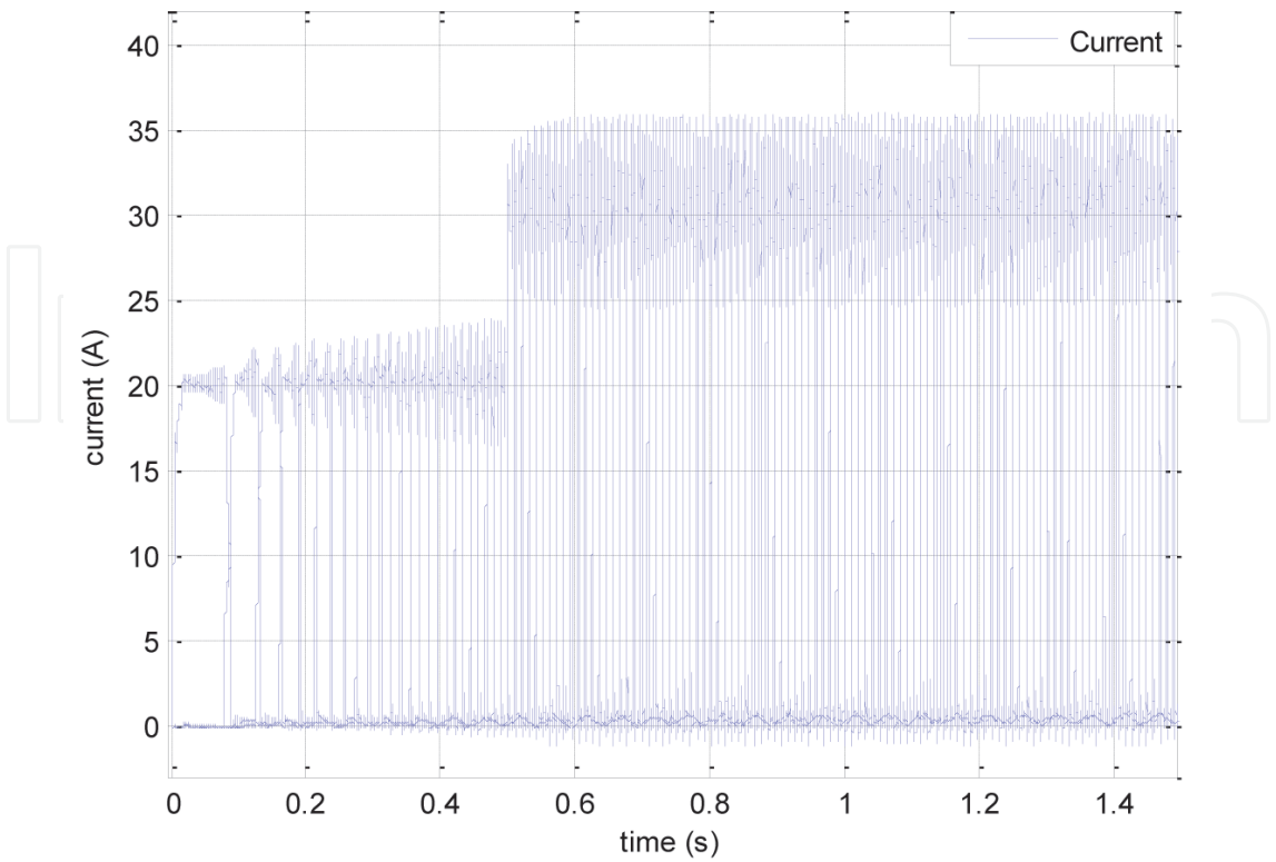
Figure 16. SRM current.
