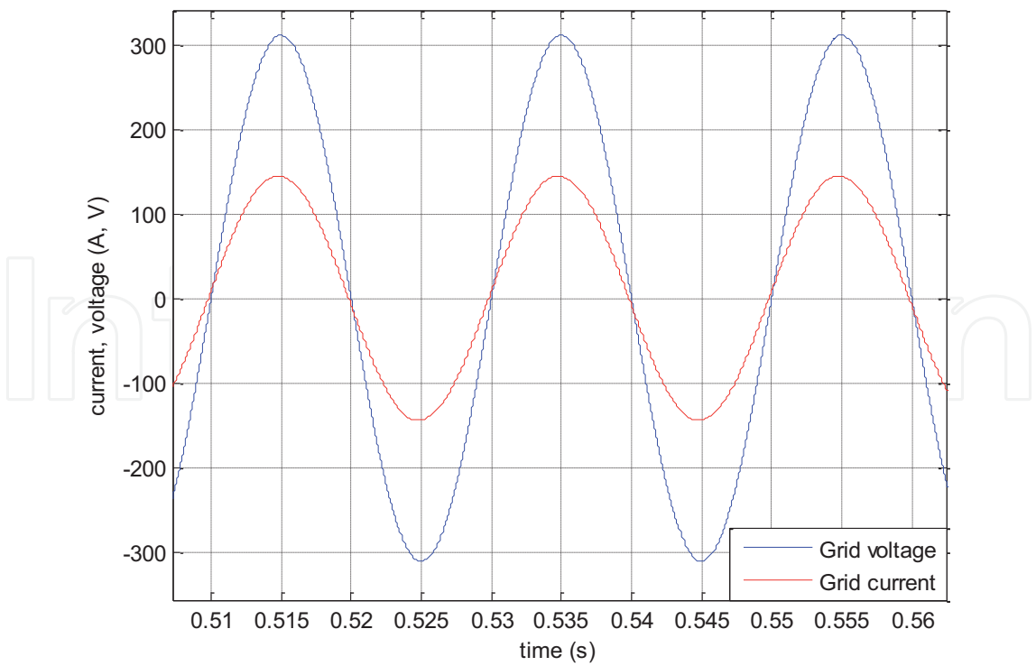
Figure 19. Single-phase current and voltage of grid.
