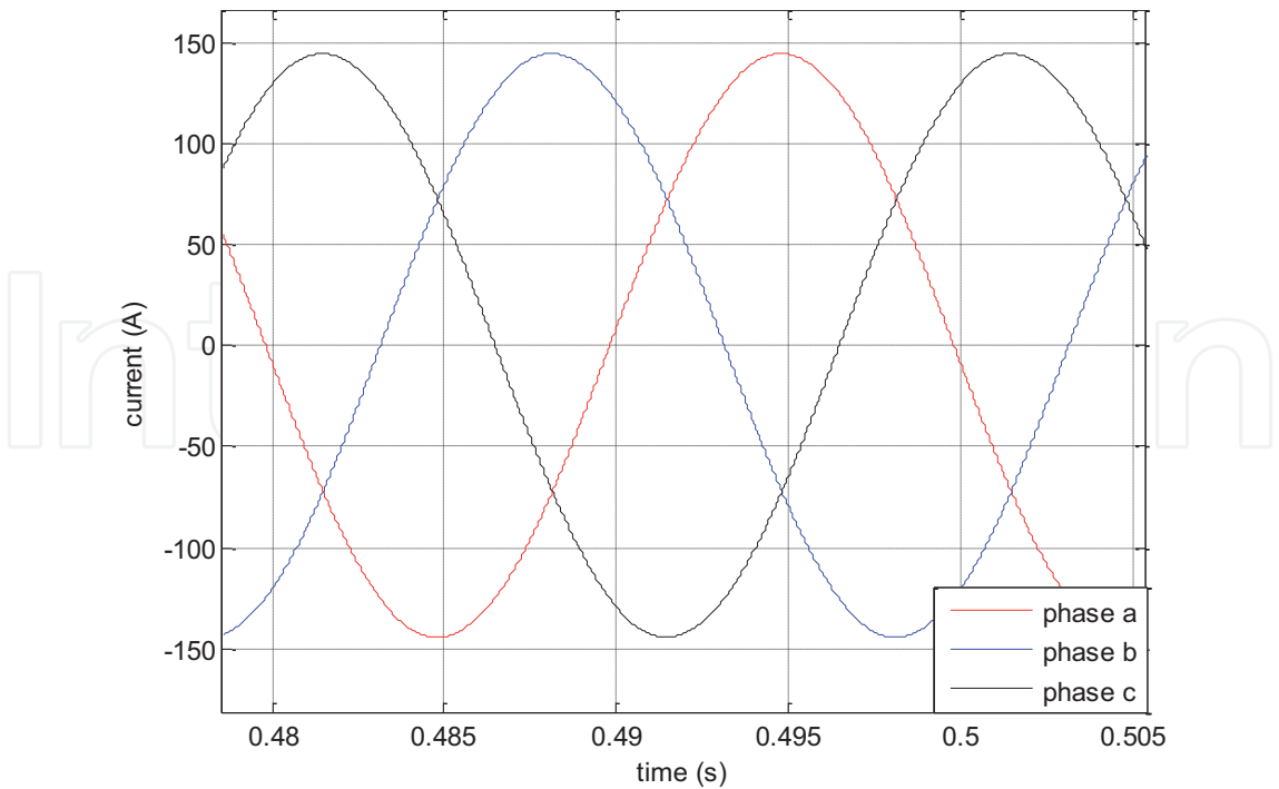
Figure 20. Three-phase currents of grid.
