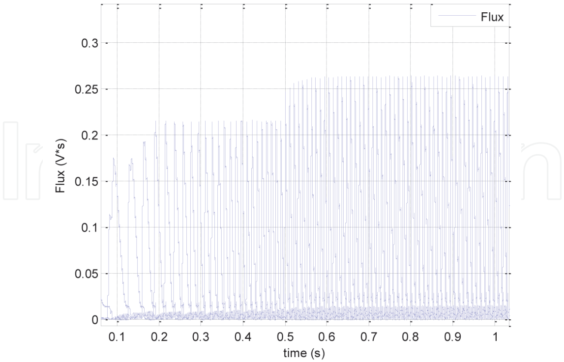
Figure 17. SRM flux.
