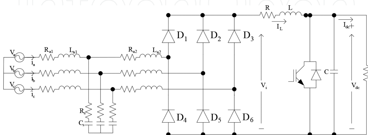
Figure 11. A three-phase PFC boost converter.
