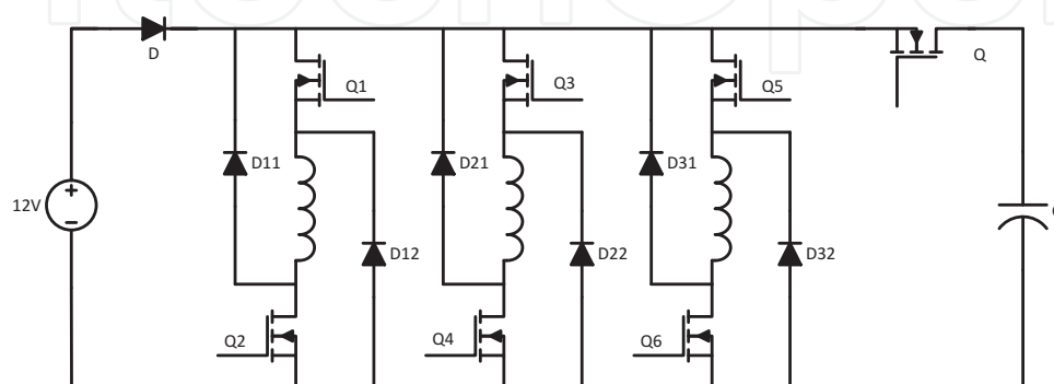
Figure 8. Proposed SRM boost converter.
