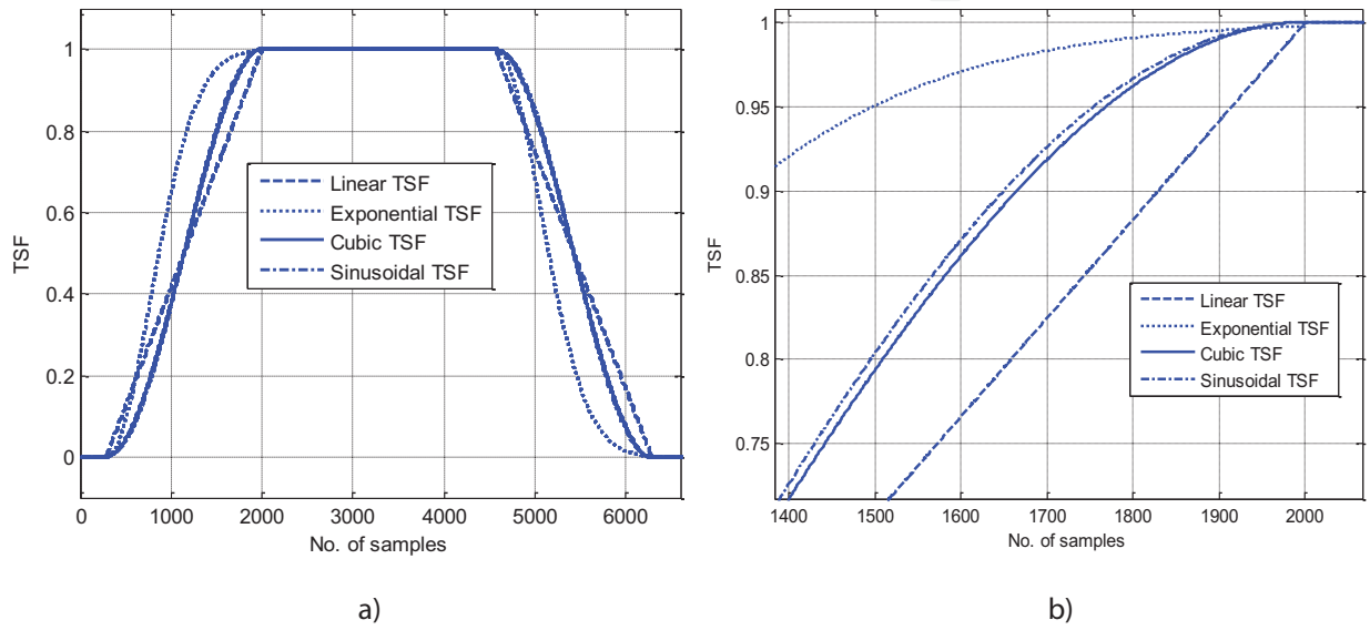
Figure 5. The variation of the TSFs used in the SRM controller.
