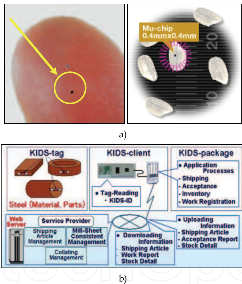
Fig. 19. Hitachi's RFID \mu -chip a) in comparison with the human finger and rice grain, and b) their application for steel-based parts' tracking
