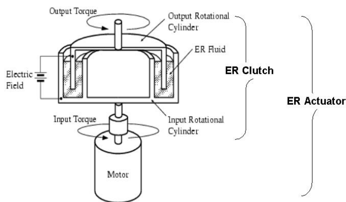
Fig. 1. Conceptual illustration of ER actuator
