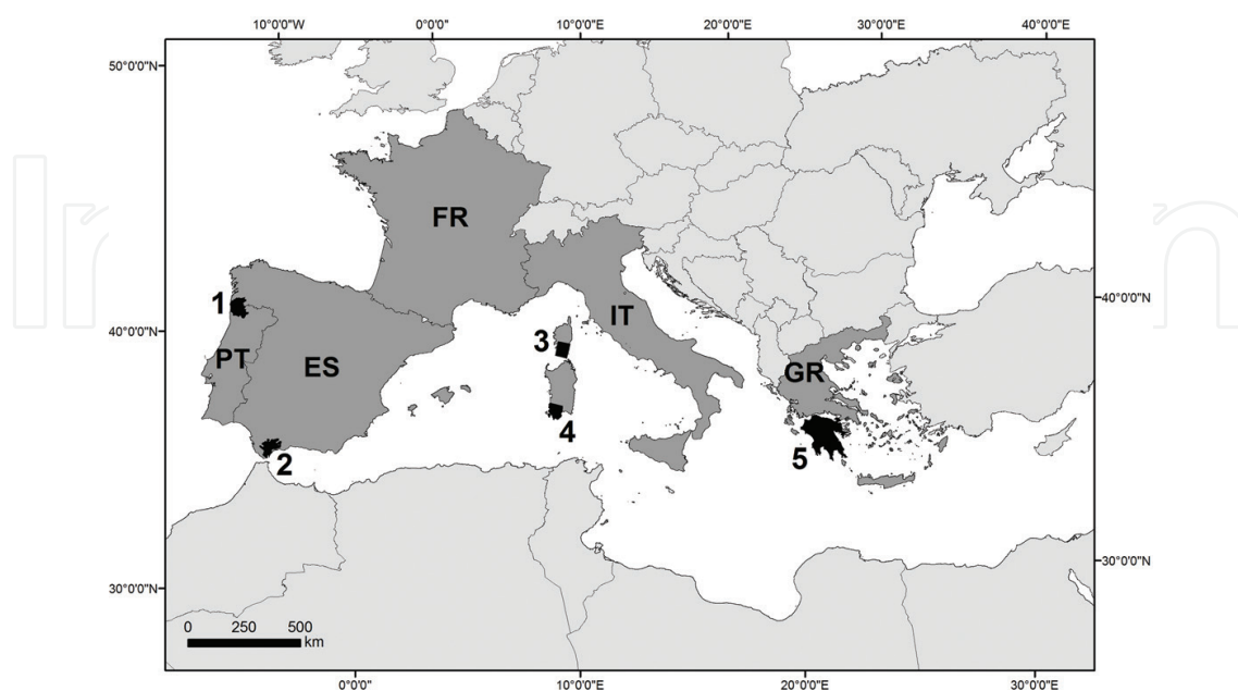
Figure 2. Geographic coverage of the PREFER project and location of the test areas in the participating countries. 1-Minho region, Portugal (PT); 2-Los Alcornocales, Andaluzia, Spain (ES); 3-SW Corsica, France (FR); 4-SW Sardinia, Italy (IT); 5-Peloponnese region, Greece (GR).
