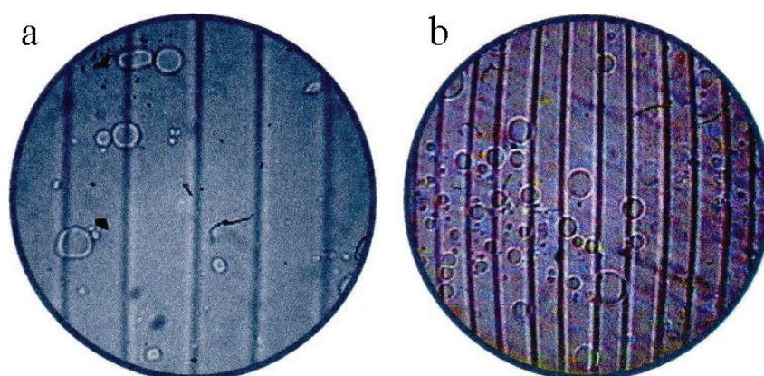
Figure 2. TEM images of hydrophobic MTX liposomes prepared by reverse-phase evaporation method: PC:MTX = 10:1 (a), PC:CH:MTX = 10:1:1 (b).
