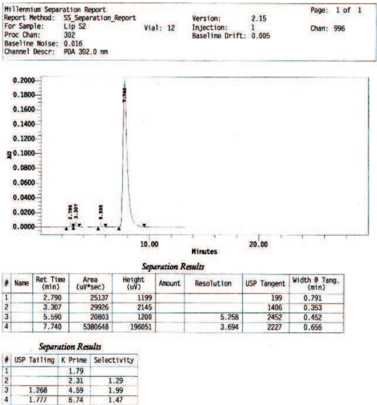
Figure 12. Chromatogram of hydrophobic methotrexate liposomes.
