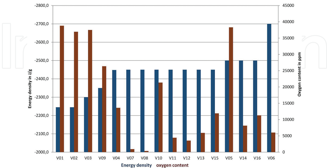
Figure 4. The various aluminothermic trials of the mechanically activated rutile for 2 h and CaO 2 as a booster.
