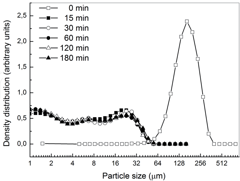
Figure 9. Grain size distributions of FeTiO 3 /Al mixtures with various times of mechanical activation.
