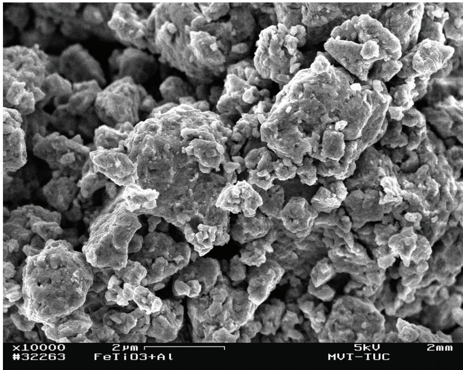
Figure 10. SEM image of formed FeTiO 3 /Al agglomerates.
