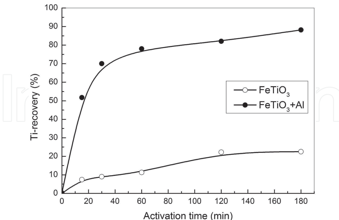
Figure 11. Influence of mechanical activation time of FeTiO 3 and FeTiO 3 /Al mixtures on Ti extraction during 60 min of leaching.
