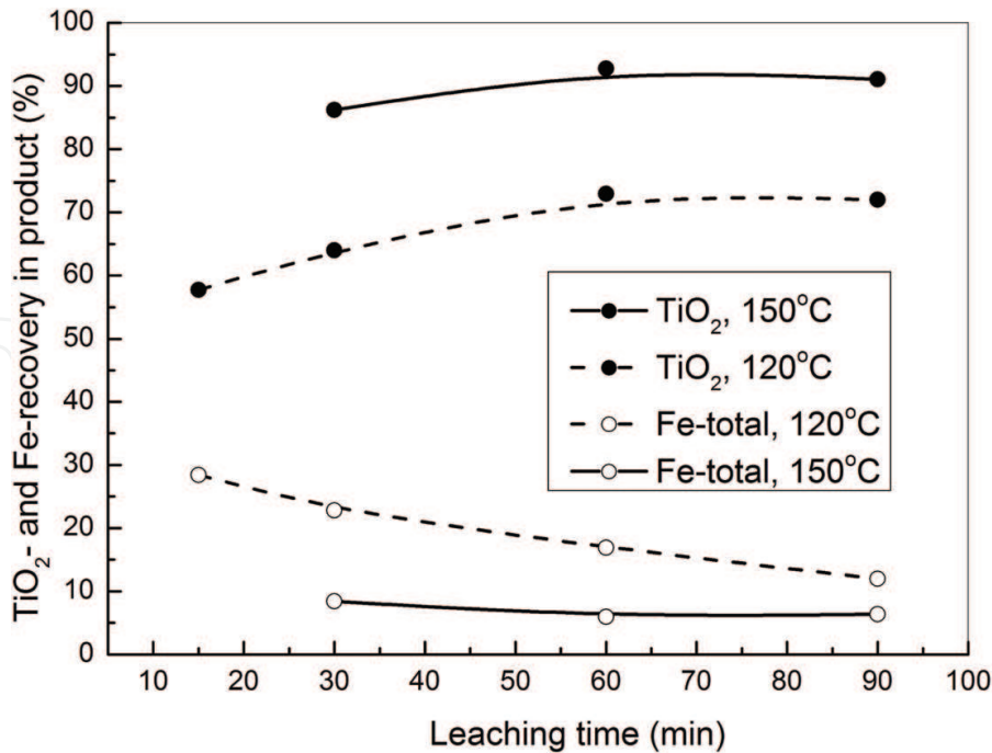
Figure 7. Influence of the leaching time and the temperature on the precipitation of \text{TiO}_2 ; s/l ratio: 50 \text{ g.l}^{-1} , mechanical activation time: 15 min, \text{H}_2\text{SO}_4 : 30%, and Fe powder: 6%.
