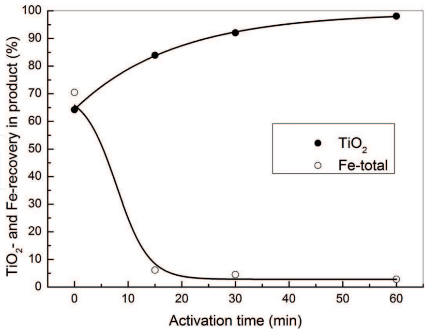
Figure 6. Influence of the mechanical activation time of \text{FeTiO}_3 on the precipitation of \text{TiO}_2 ; leaching temperature: 150^\circ\text{C} , s/l ratio: 50 \text{ g.l}^{-1} , leaching time: 60 min, \text{H}_2\text{SO}_4 : 30%, and Fe powder: 12%.
