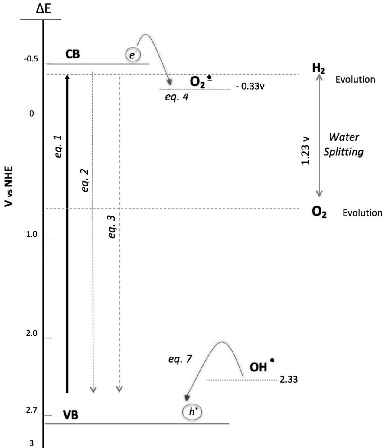
Figure 2. TiO 2 potential energy and ROS reaction generation to normal hydrogen electrode at pH = 7.0 (NHE) [20–22].
