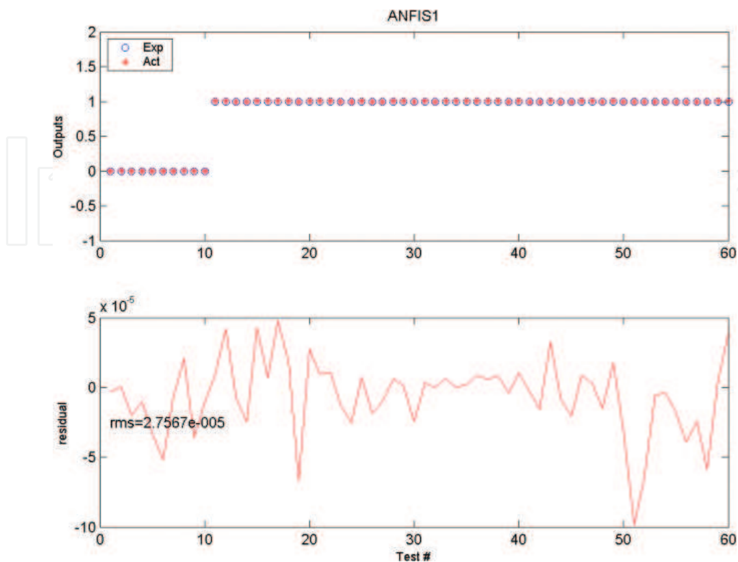
Figure 6. Testing results and the corresponding error curves (ANFIS1, ANFIS-2D-WT method, using all six sensors).
