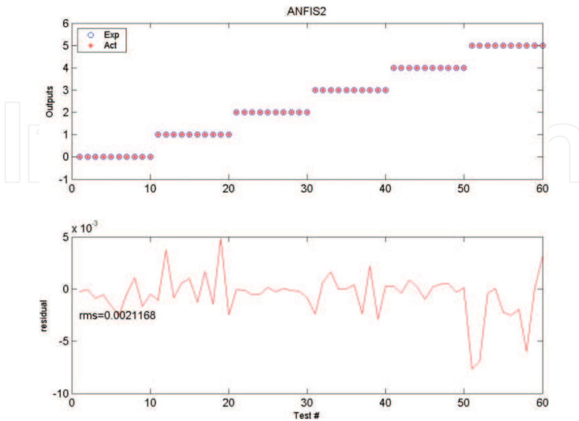
Figure 8. Testing results and the corresponding error curves (ANFIS2, ANFIS-2D-WT method, using all six sensors).
