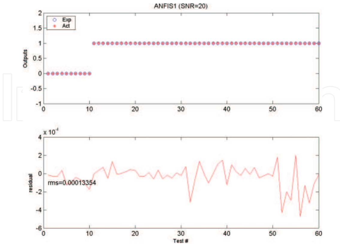
Figure 9. Testing results and the corresponding error curves (ANFIS1, ANFIS-2D-WT method, SNR = 20).
