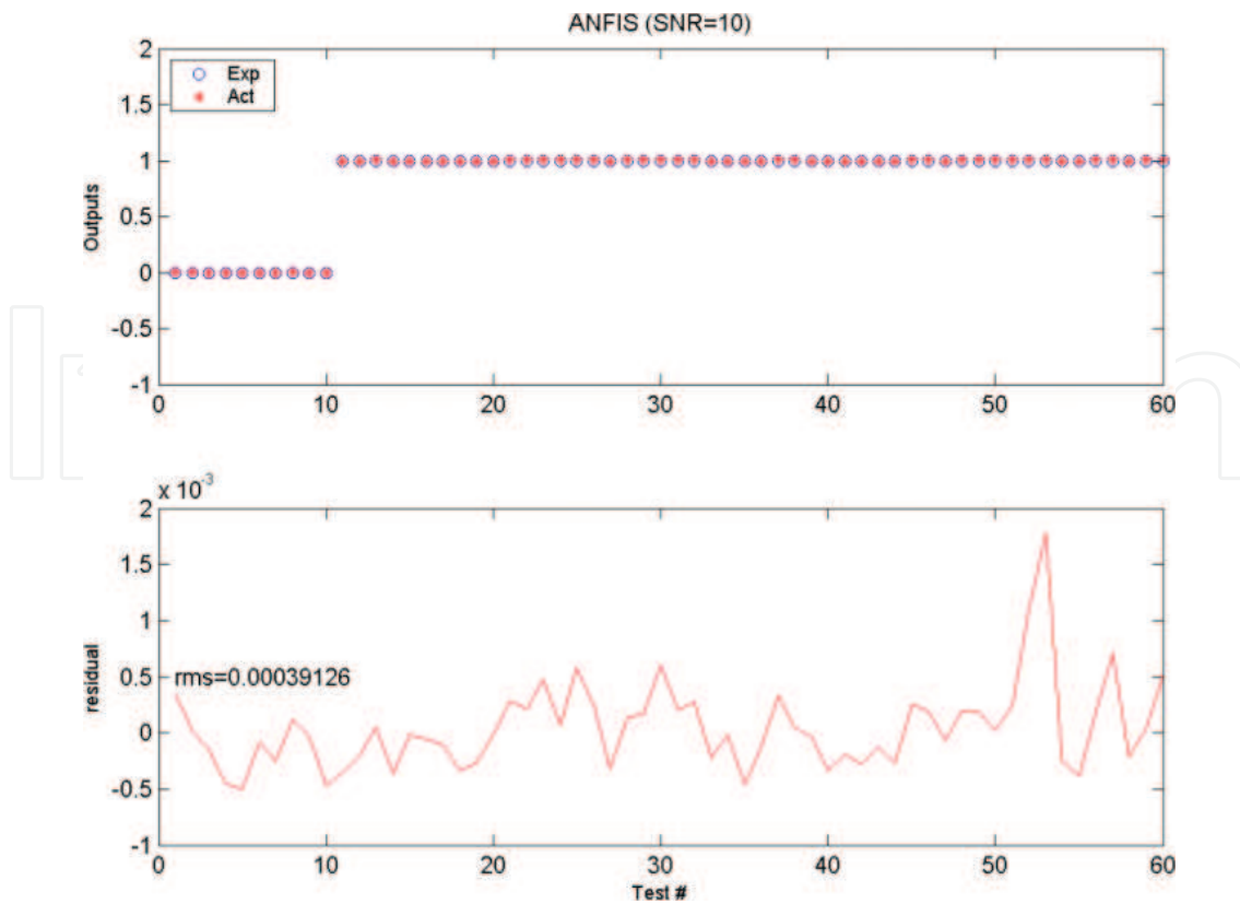
Figure 10. Testing results and the corresponding error curves (ANFIS1, ANFIS-2D-WT method, SNR = 10).
