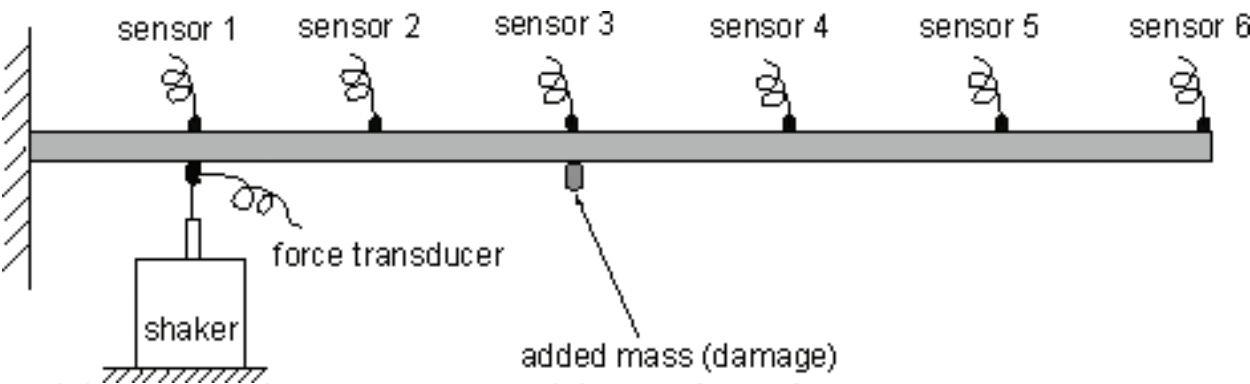
Figure 4. Cantilever beam experiment; setup schematic representation.
