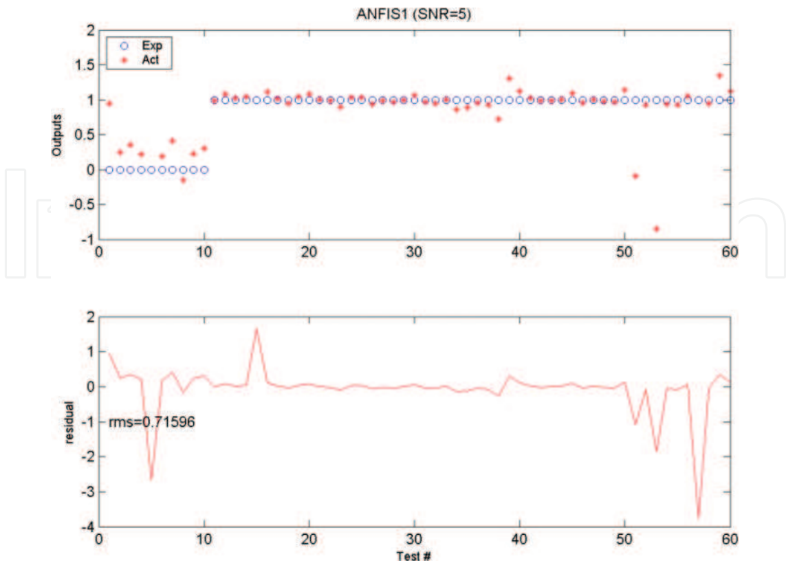
Figure 11. Testing results and the corresponding error curves (ANFIS1, ANFIS-2D-WT method, SNR = 5).
