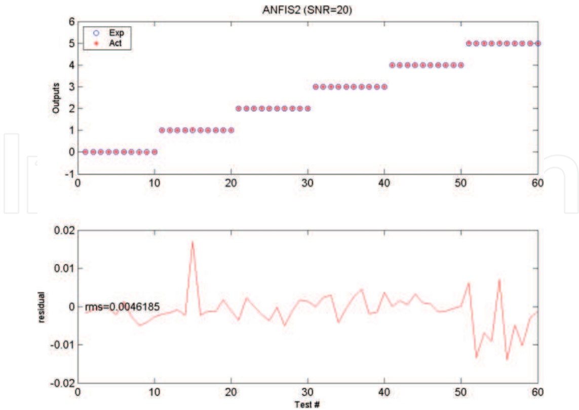
Figure 12. Testing results and the corresponding error curves (ANFIS2, ANFIS-2D-WT method, SNR = 20).
