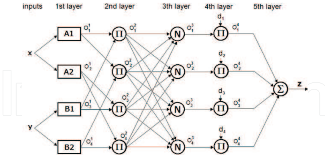
Figure 3. ANFIS architecture for a two-input Sugeno fuzzy model with four rules (from ANN point of view).
