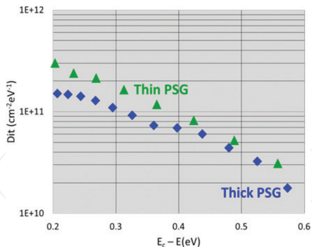
Figure 7. D_{it} for thin PSG MOS capacitor. D_{it} is lower than NO device, but higher than thick PSG device.
