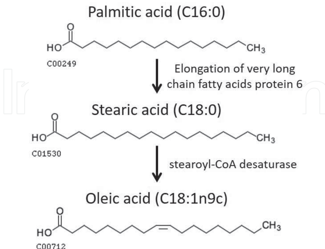
Figure 2. Schematic of palmitic and oleic acid biosynthesis pathway derived from KEGG pathway maps [2].
