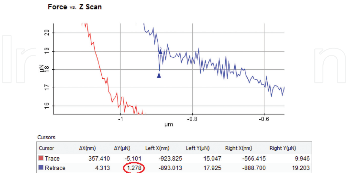
Figure 9. Adhesion force between the central part of micromembrane and the substrate in the case of micromembrane with 2 \times 4 connected hinges.
