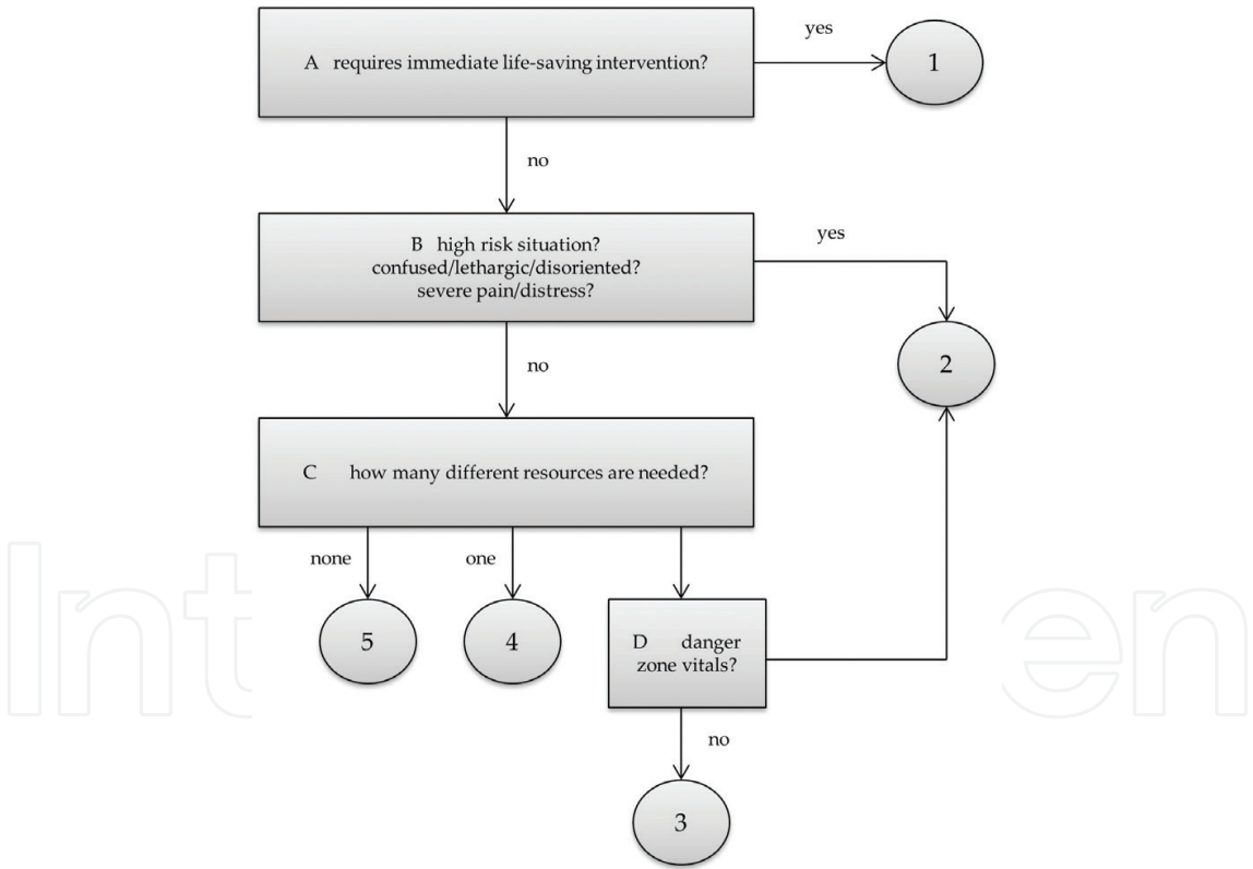
Figure 2. ESI approach.
