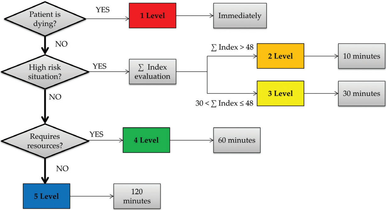
Figure 4. TAEM approach.
