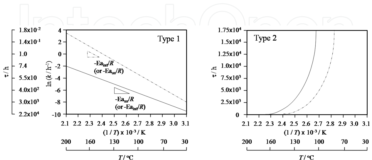
Figure 7. Two different types of \tau - T diagrams.
