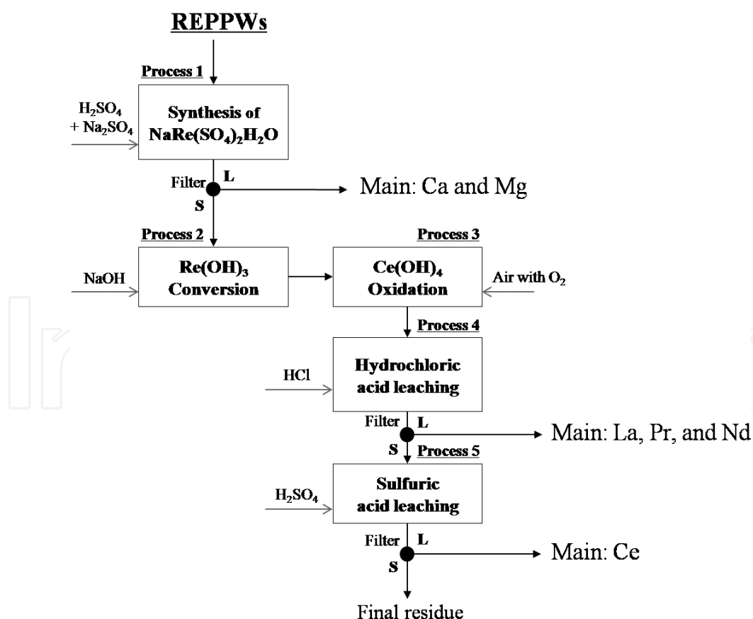
Figure 4. Schematic flow diagram for separation of rare earth elements from rare earth polishing powder wastes via a devised hydrometallurgical process (Um and Hirato, 2016) [16].
