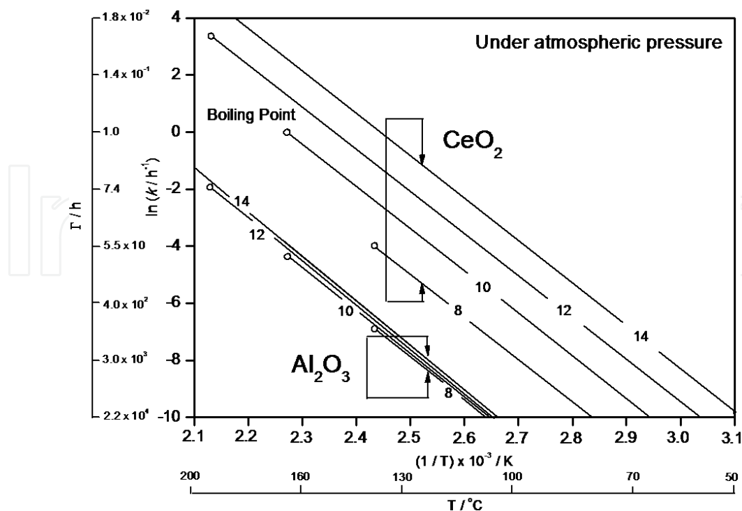
Figure 9. Revised \tau - T diagram for \text{CeO}_2\text{-Al}_2\text{O}_3\text{-H}_2\text{SO}_4\text{-H}_2\text{O} system (Um and Hirato 2013) [14].
