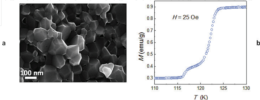
Figure 5. (a) SEM micrograph of magnetite consolidated by SPS at 750°C, 15 min and (b) magnetization measurements showing the Verwey transition (adapted from Ref. [49]).
