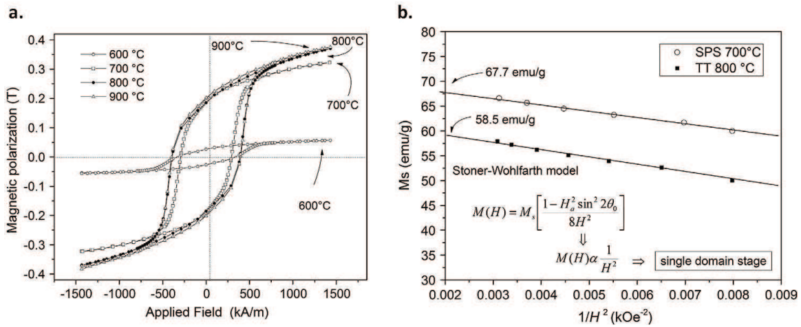
Figure 10. Sr-Fe 12 O 19 prepared by SPS-assisted mecnosynthesis: (a) Hysteresis loops M vs H showing the effect of the SPS temperature on the magnetic properties and (b) comparison of the saturated magnetization M_s vs 1/H^2 obtained after either SPS heating or conventional annealing. Republished with permission from Ref. [65] Copyright 2014, with permission through Copyright Clearance Center, Inc., Elsevier.
