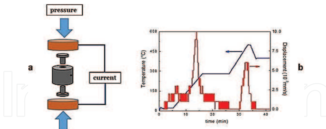
Figure 2. (a) SPS electrodes and die set up; (b) a typical temperature profile (left axis), and shrinkage trace (right axis), in the form of time derivative dZ/dt for a spinel ferrite (adapted from Ref. [7]).
