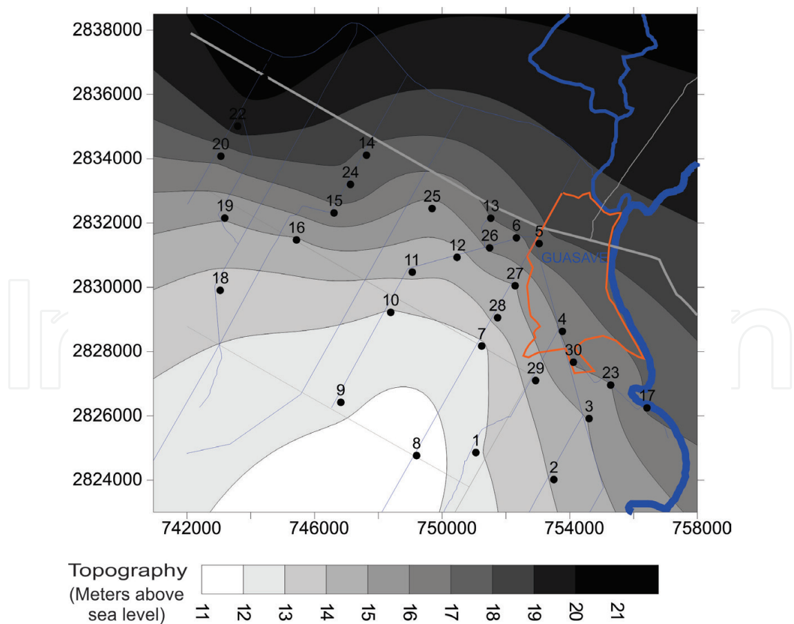
Figure 2. Topographic relief of the study area.
