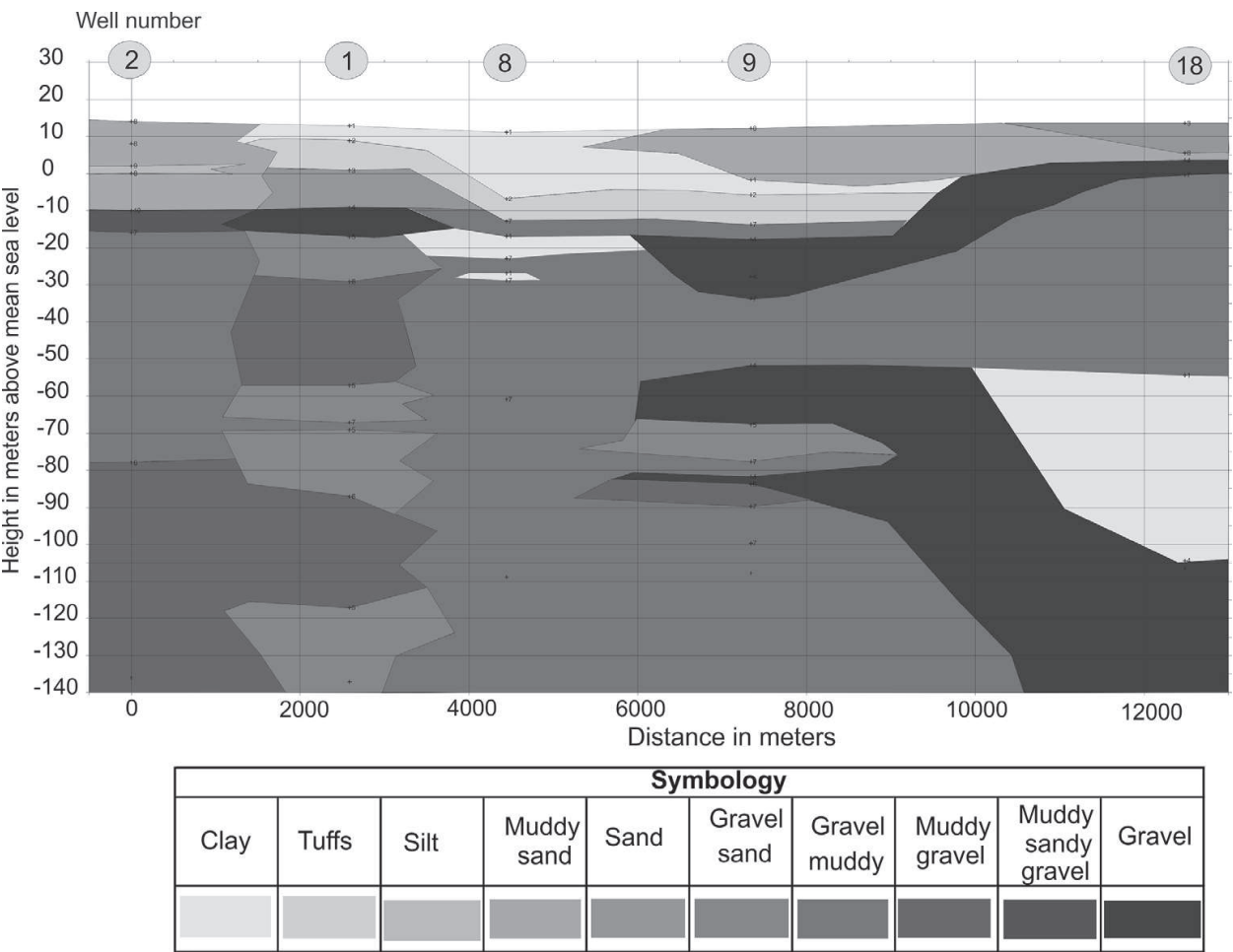
Figure 3. Section perpendicular to the Sinaloa River.
