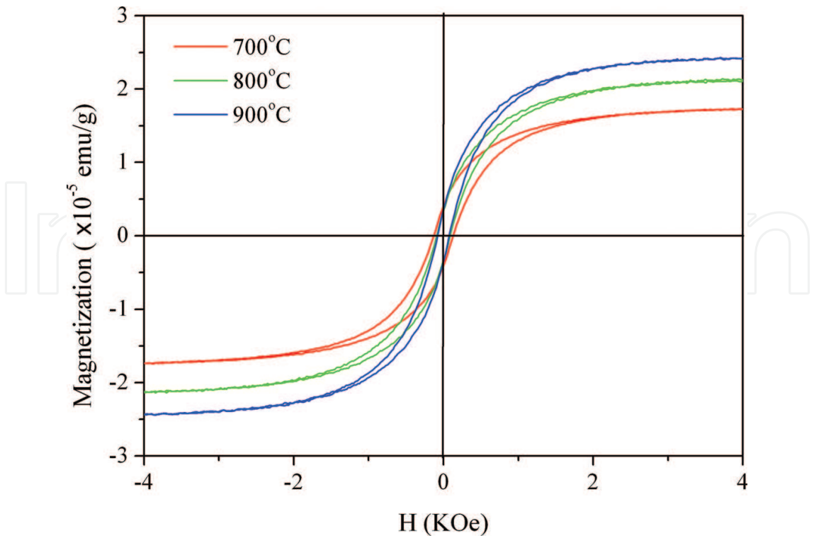
Figure 17. M-H loops at 300 K of sample implanted at dose 3 \times 10^{16} ions \text{cm}^{-2} and annealed [66].
