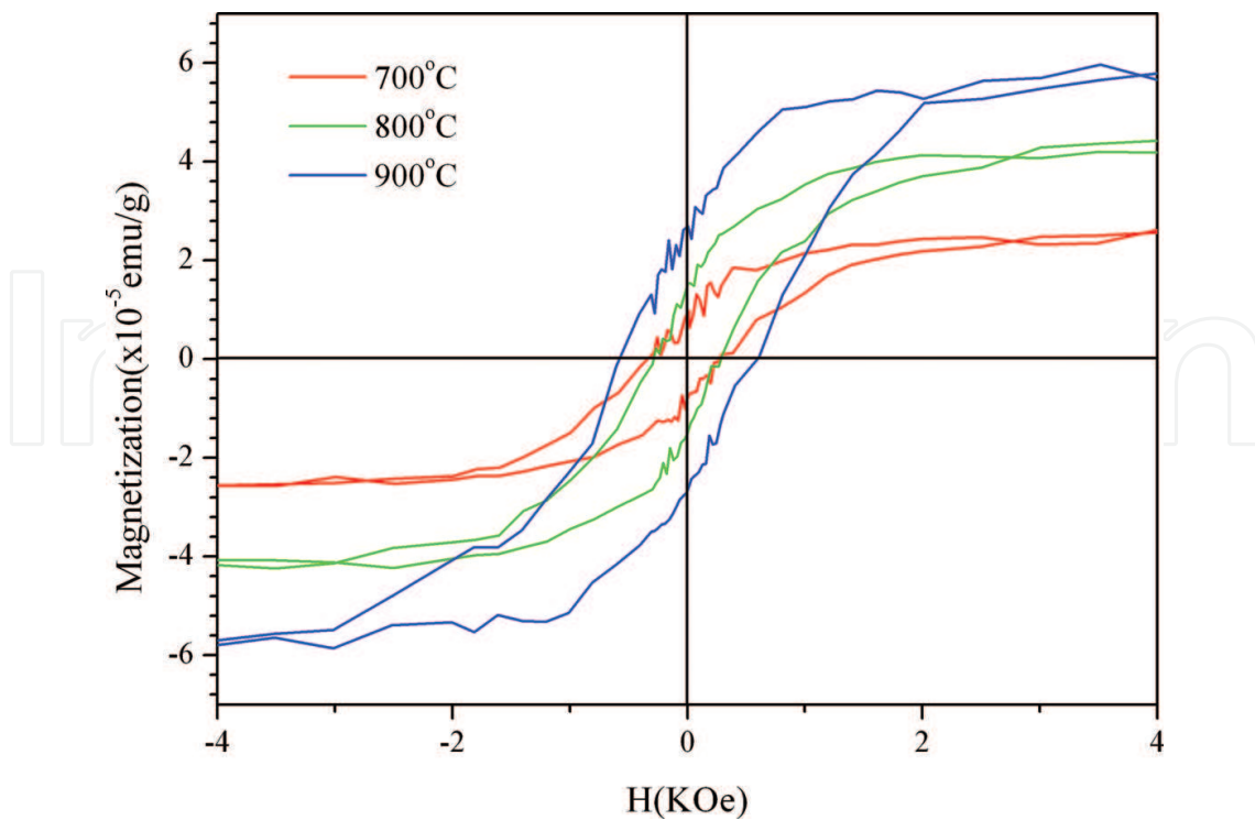
Figure 20. M-H loops at 5 K of sample implanted at dose 5 \times 10^{16} ions cm -2 and annealed [67].
