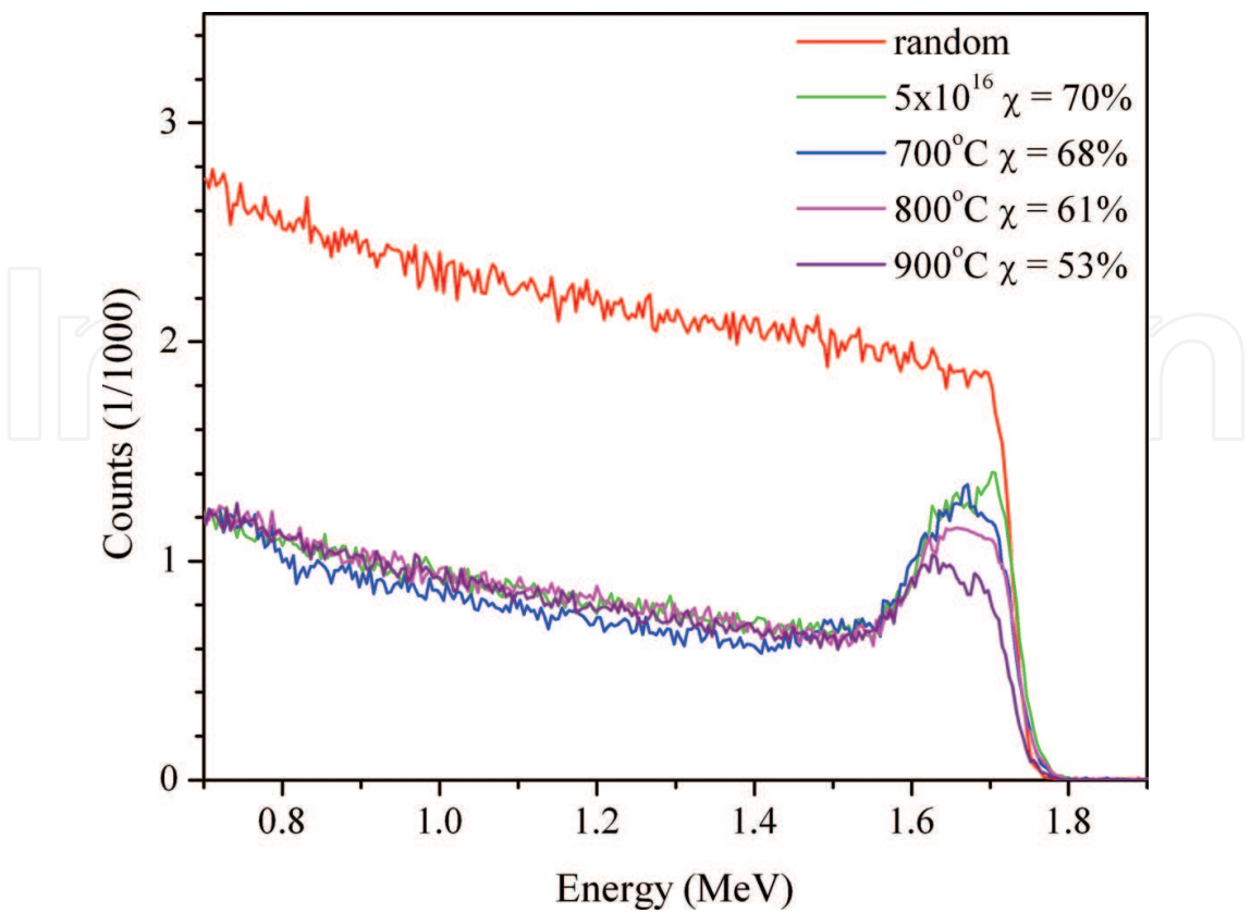
Figure 16. RBS/C of Co+ implanted GaN at 5 \times 10^{16} ions \text{cm}^{-2} and annealed samples at different temperatures [67].
