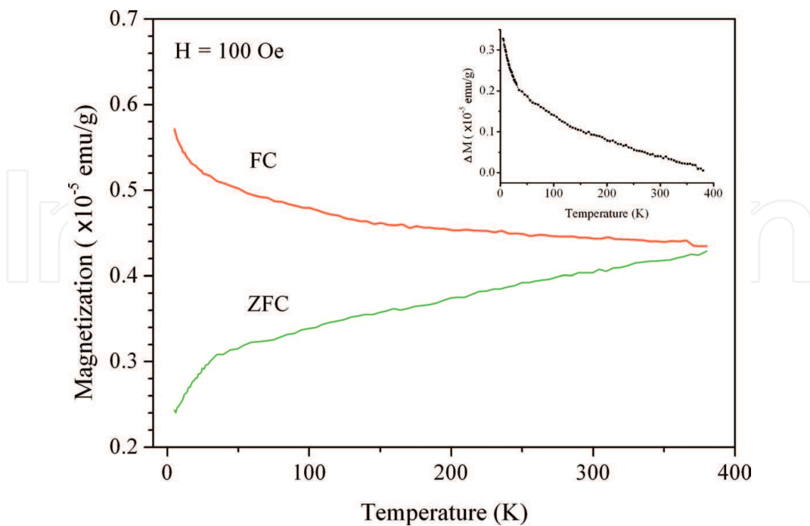
Figure 21. FC/ZFC measurements of sample implanted at a dose of 3 \times 10^{16} ions cm -2 and annealed at 900°C [66].
