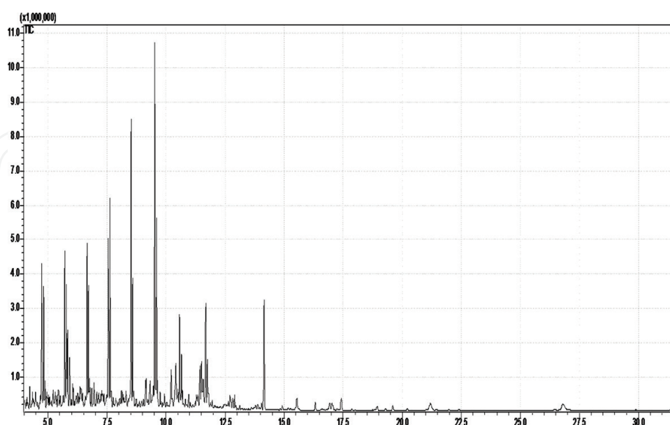
Figure 9. GC-MS of OLP obtained by catalytic cracking of palm oil at 450°C and 1.0 atm, with 15% (wt) \text{Na}_2\text{CO}_3 in pilot scale.
