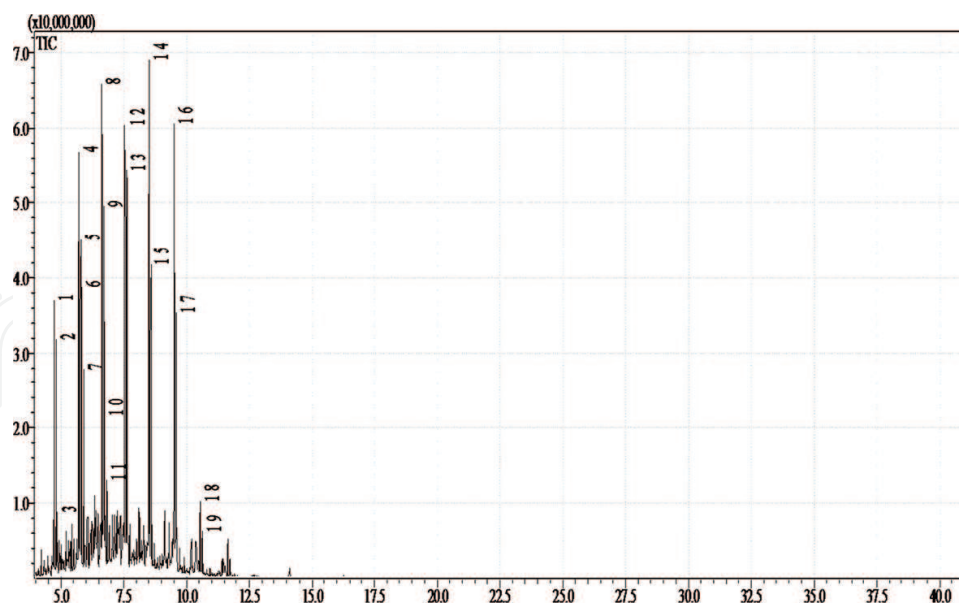
Figure 10. GC-MS of light diesel-like hydrocarbon fraction produced in a pilot-packed distillation column with internal reflux of 100 cm height with OLP obtained at 450°C and 1.0 atm, with 15% (wt) \text{Na}_2\text{CO}_3 in pilot scale.
