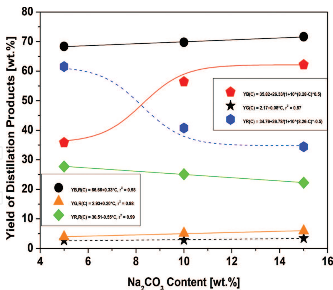
Figure 3. Yield of distillation products (distillates, bottoms, and gas), produced by laboratory distillation with (YB,R, YR,R, and YG,R) and without reflux (YB, YR, and YG) with OLPG obtained at 450°C and 1.0 atm, with 5, 10, and 15% (wt) Na 2 CO 3 in pilot scale, using a column of 50 cm.
