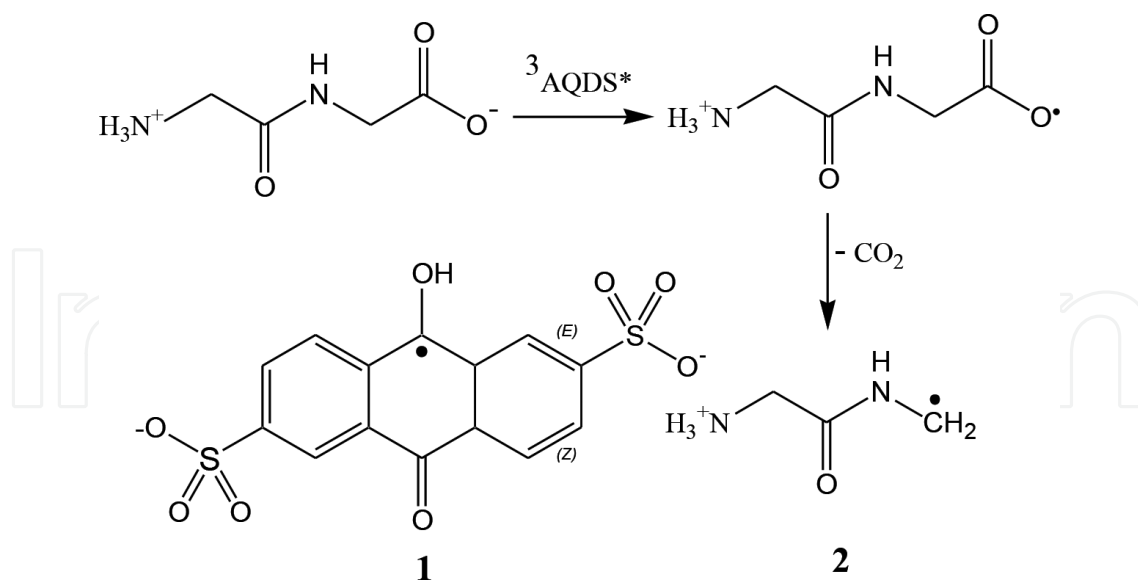
Scheme 7. Generation of geminate triplet radical pair 1...2 under the photolysis of AQDS in AOT reverse micelles.
