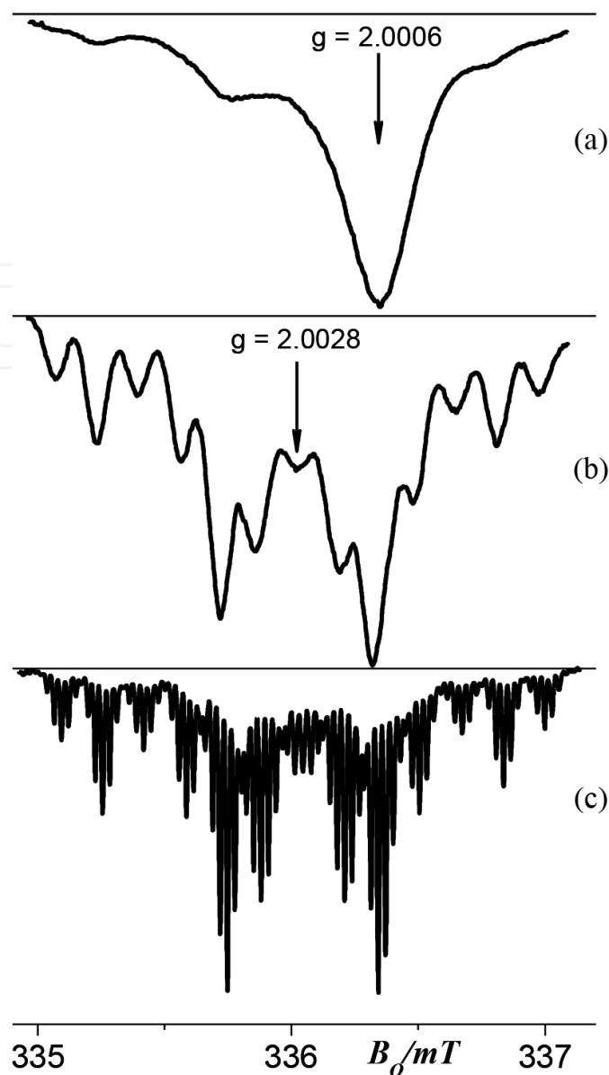
Figure 2. TREPR spectra at t_{\text{obs}} = 260 ns (a), = 1.12 \mu\text{s} (b), and = 3.6 \mu\text{s} (c) of geminate radical pairs resulting from photodissociation of Irgacure ® 651 ( Scheme 1 ) in micellar aqueous solutions of SDS at room temperature [40, 41].
