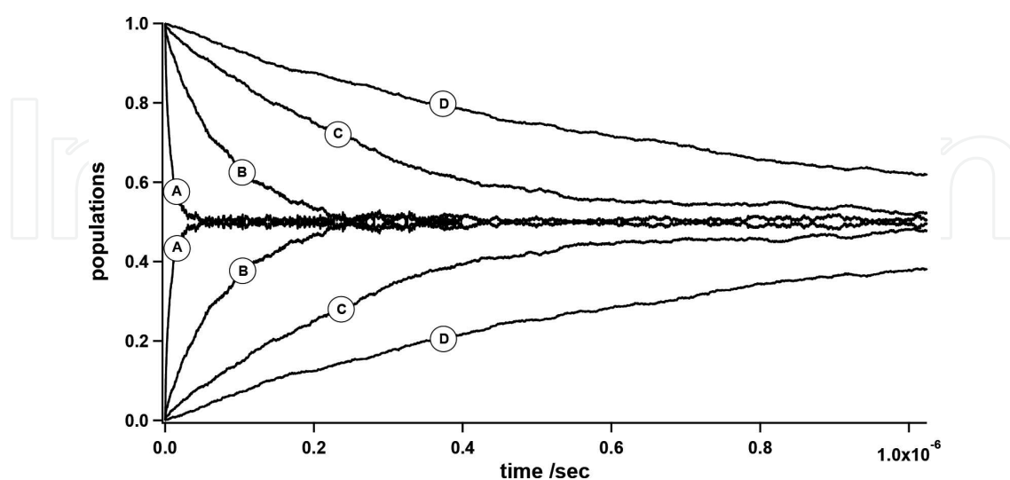
Figure 16. Relaxation of populations due to electron spin–spin exchange interaction as function of micelle size. L_m = 16 \text{ \AA} (A), 32 \text{ \AA} (B), 48 \text{ \AA} (C), and 64 \text{ \AA} (D). Both radicals diffuse, no escape, no chemical reaction, J_0 = -2 \times 10^{10} \text{ rad/s} ; \lambda = 0.5 \text{ \AA} ; D_a = D_b = 10^{-6} \text{ cm}^2 .
