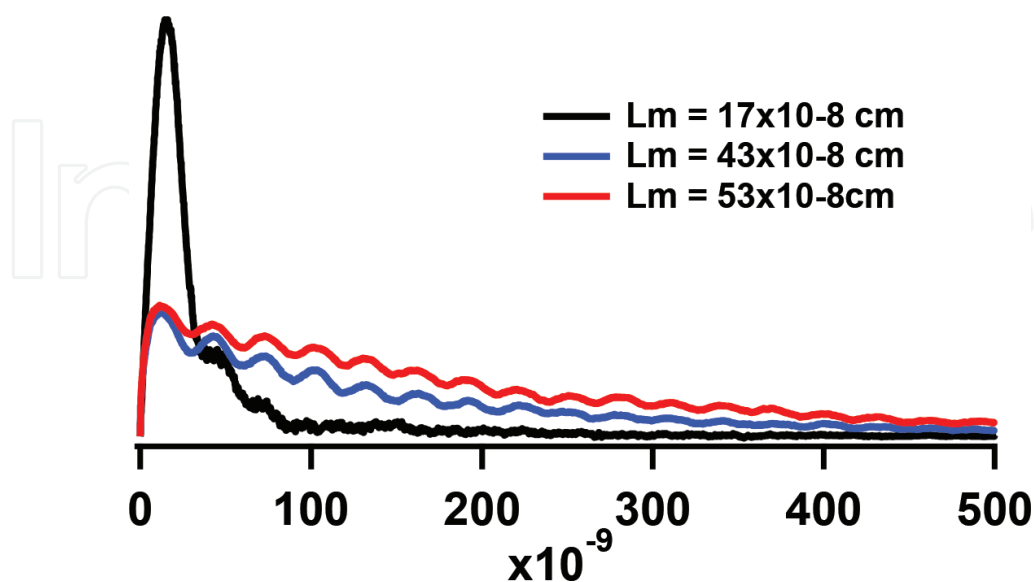
Figure 15. Generation and decay over time of the ST 0 RPM polarization in AOT reverse micelles. Water core radii are given in the insertion. All other parameters are listed in Table 4 . The TM polarization is neglected.
