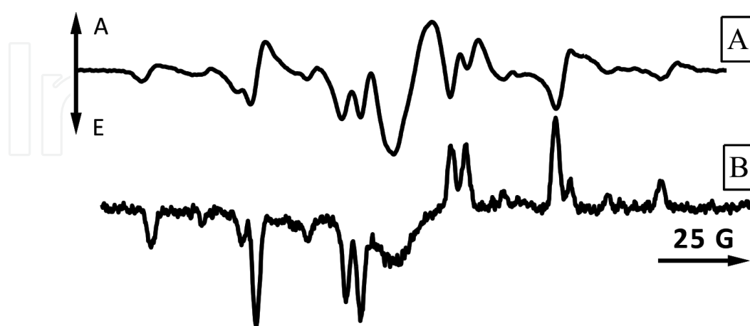
Figure 5. TREPR ( t_{\text{obs}} = 500 ns) spectra of geminate pairs \text{Alk}\cdot and \text{BPH}\cdot radicals produced in photochemical ( \lambda = 308 nm) oxidation of SDS detergent by the electronically excited triplet state of benzophenone (0.4 mM) in micellar aqueous solution of SDS (10 mM) (A) and benzophenone (0.4 mM) in ACN/ \text{H}_2\text{O} = 50:50 solution of SDS which does not contain micelles.
