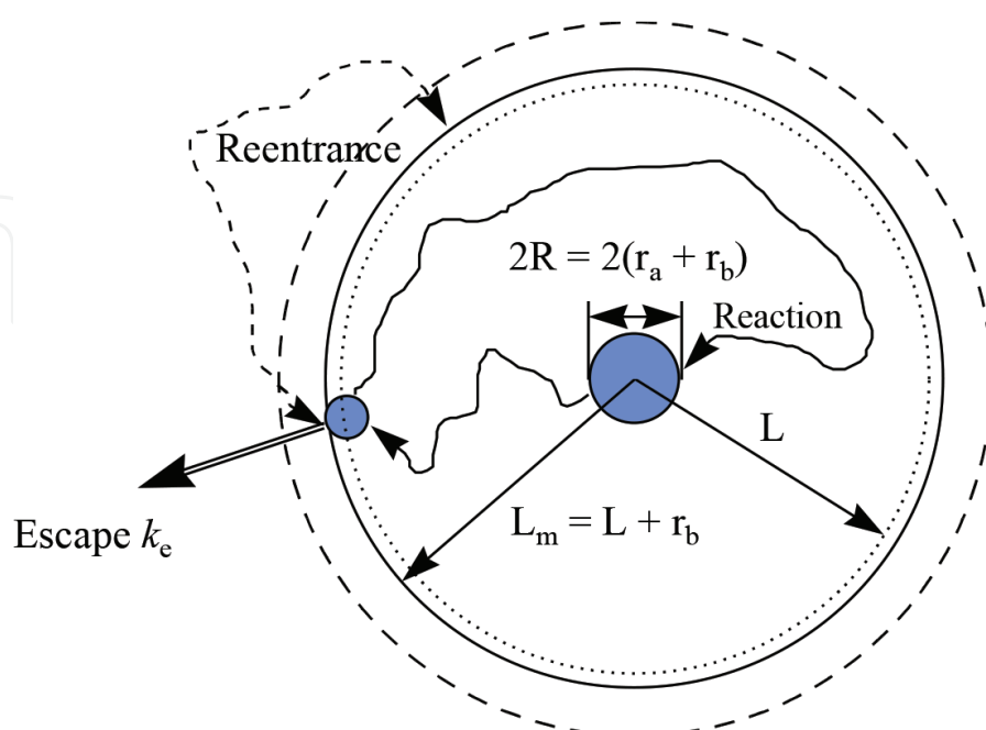
Scheme 4. Visualization of the microreactor model for SCRPs.
