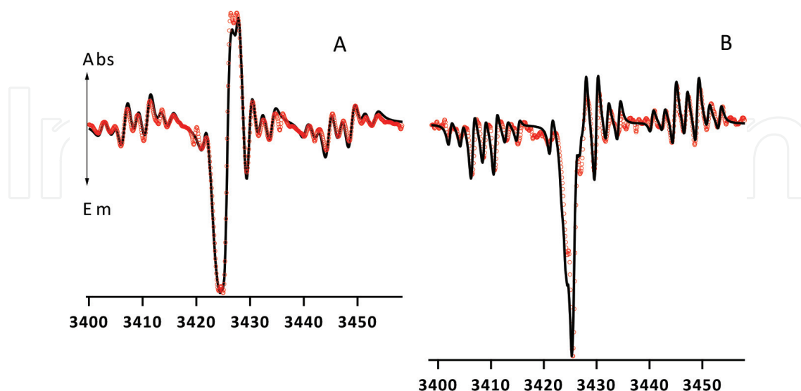
Figure 11. TREPR spectra (empty circles) observed under photooxygenation (laser flash photolysis, \lambda = 308 nm) of GG by AQDS in AOT micelles for L_m values of 23 Å (A) and 53 Å (B), at room temperature. Solid lines are simulations in terms of the microreactor model.
