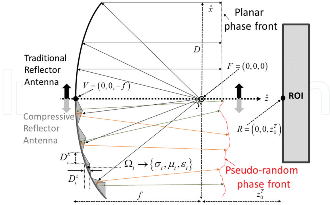
Figure 1. 2D cross-sections of a traditional reflector antenna ( x > 0 ) and a compressive reflector antenna (CRA) ( x < 0 ), where all the design parameters are described.
