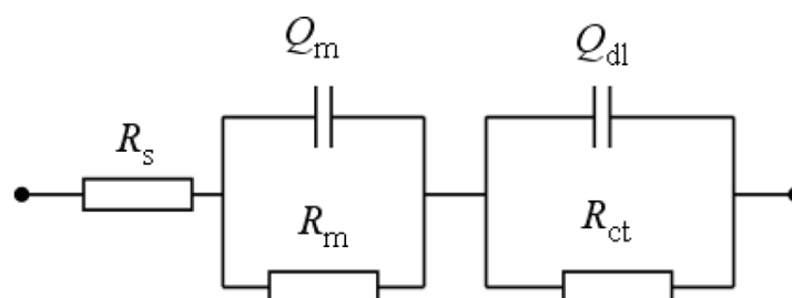
Figure 5. The equivalent circuit models used to fit the experiment impedance data of the CuO-graphene cathode in a 10 g/L \text{Na}_2\text{SO}_4 solution.
