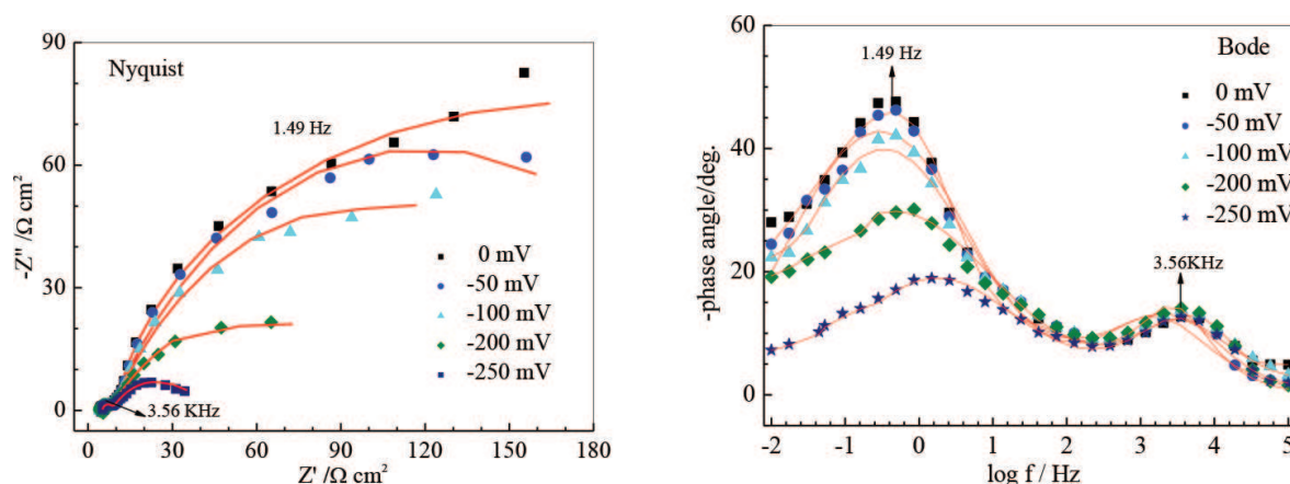
Figure 4. The experimental (dots with different symbols) and the fitted (solid lines) EIS curves of the CuO-graphene cathode according to the presented equivalent circuit immersed in a 10 g/L \text{Na}_2\text{SO}_4 solution under different reduction potentials.
