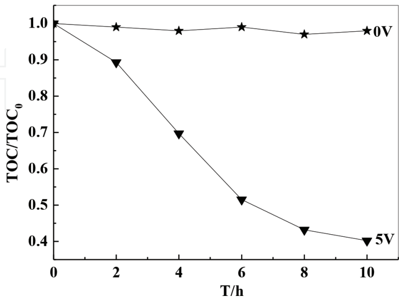
Figure 9. Evolution of TOC for the degradation of Terramycin, initial tetracycline concentration, 60 \mu\text{g/L} ; initial pH = 7.0; electrolyte, 10 g/L \text{Na}_2\text{SO}_4 .
