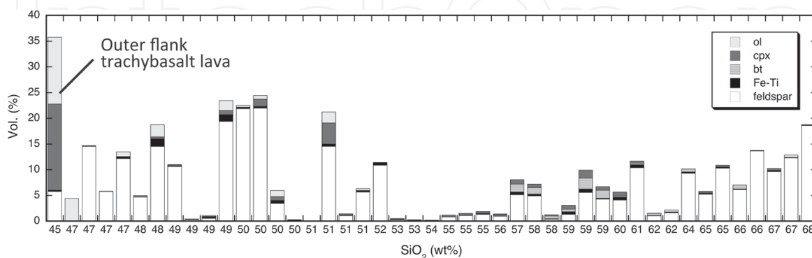
Figure 5. Variations in phenocryst type and abundance with changing \text{SiO}_2 concentration within the ODS rocks (modified after Ref. [16]). Abbreviations: ol: olivine; cpx: clinopyroxene; bt: biotite; Fe-Ti: Fe-Ti oxide minerals; feldspar: plagioclase and/or potassium feldspar.
