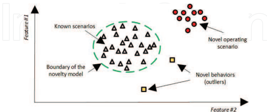
Figure 2. Example of a novelty detection basic operation, including available data, \Delta , mathematical description of the available data, --, novel behaviors detected as outliers, \square and novel behaviors detected as the novel operating scenario, O .
