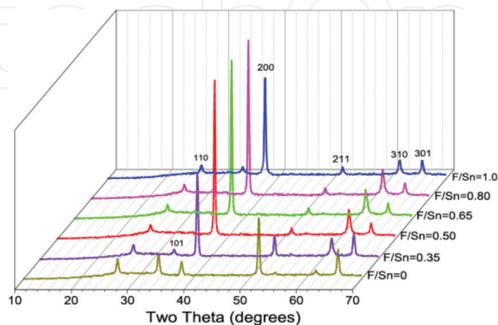
Figure 2. XRD spectra of FTO films with a thickness of around 500 nm and different F/Sn ratios in the precursor.
