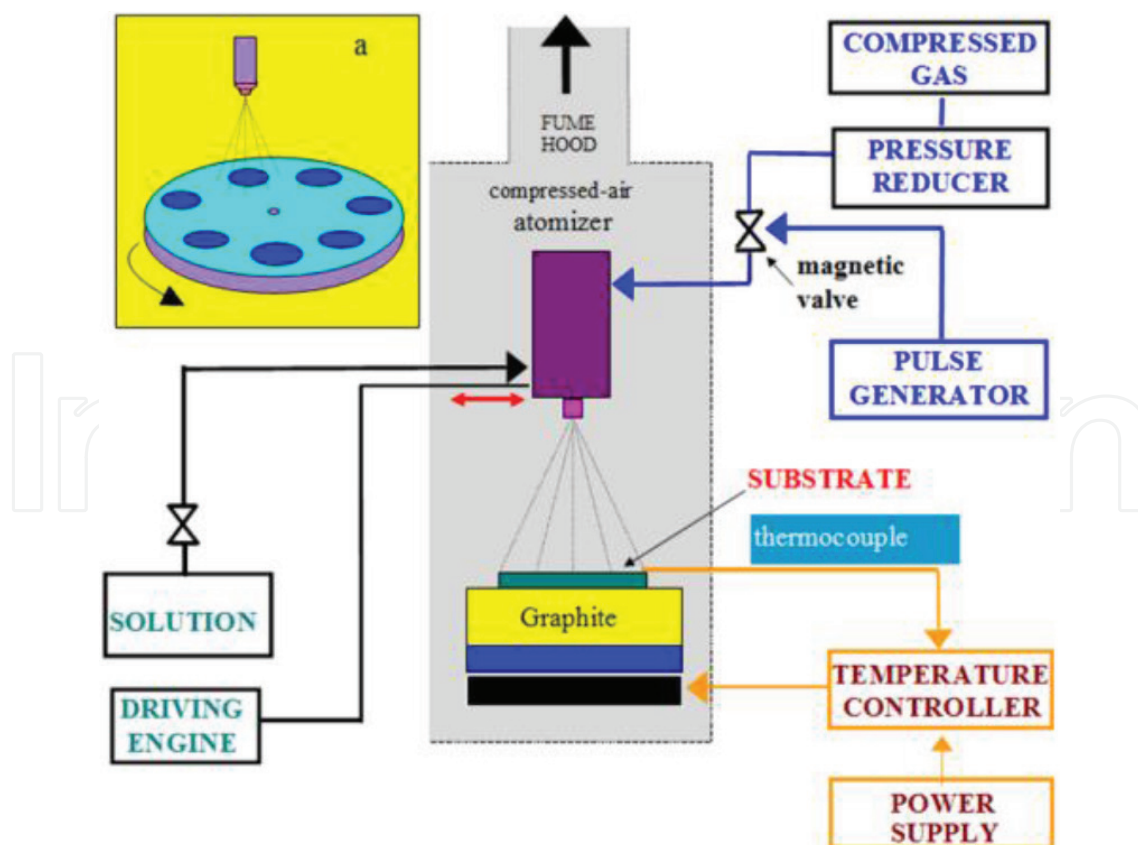
Figure 1. Schematical representation of our spraying system.
