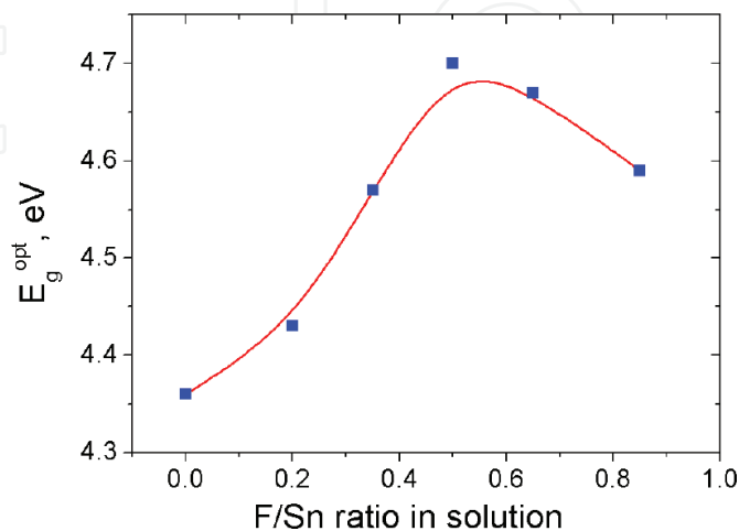
Figure 7. Value of the optical gap for FTO films fabricated from the solutions with different F/Sn ratios.
