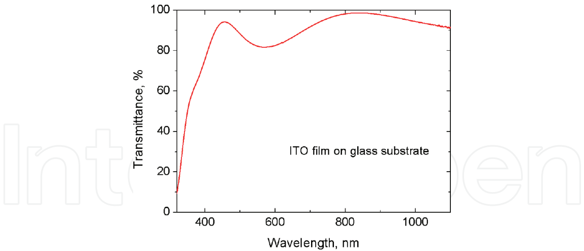
Figure 9. Transmittance of the ITO films fabricated using an indium acetate solution with a Sn/In= 6 at.% ratio.
