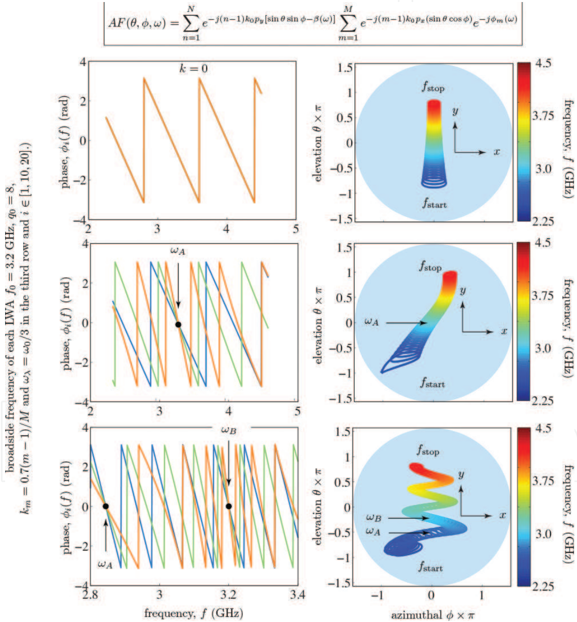
Figure 9. Array factor computed results corresponding to the structure in Figure 8 with M \times N = 20 \times 30 showing the dispersion profile of the phaser feeding elements at the input of each leaky-wave antenna and the 3-dB contour plots of the 2D radiation patterns in the (\theta, \varphi) plane [19]. ©IEEE; reprinted with permission.
