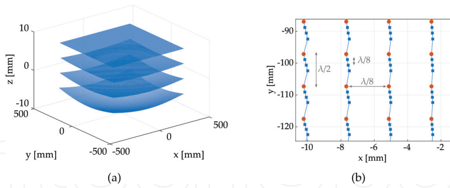
Figure 4. Three-dimensional acquisition grid for the proposed method. Note that a different scale has been used for all the axes: (a) complete grid and (b) detail of the top view.
