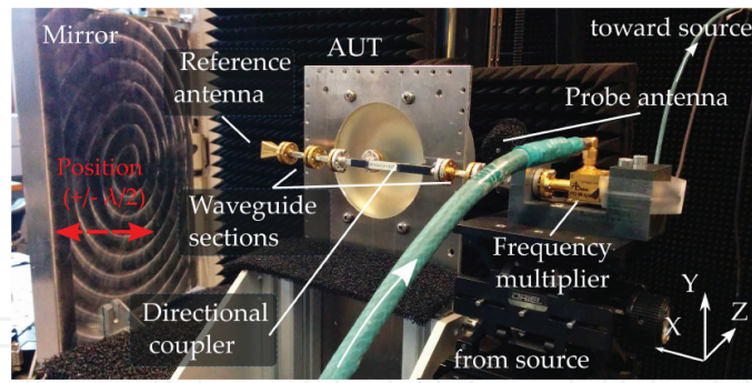
Figure 9. Measurement setup for the lens antenna characterization at 94 GHz. Rear view.
