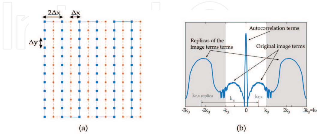
Figure 8. (a) Spatial multiplexation of the subsampled grids for the hologram formation. (b) Spectrum of the hologram for the proposed method for an example with \Delta x = \lambda/6 sampling.
