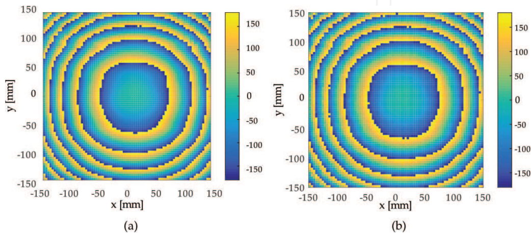
Figure 15. Retrieved phase of the AUT at 30 GHz compared to the direct measurement: (a) directly acquired phase in the NF, degrees, and (b) retrieved phase, degrees.
