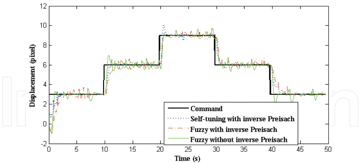
Figure 11. Multi-step input response by different control schemes.
