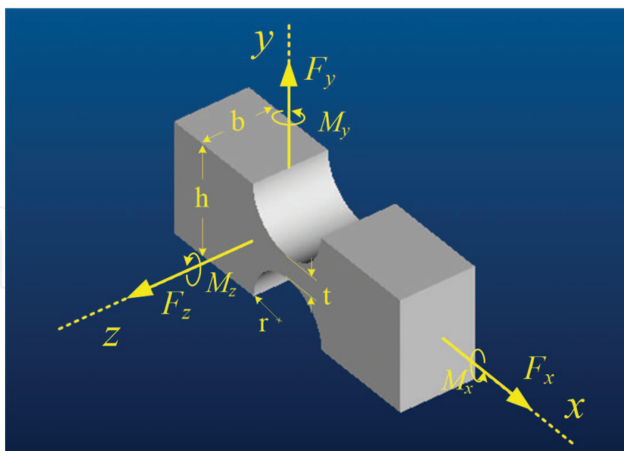
Figure 2. Geometrical dimensions and loadings of a right circular joint.
