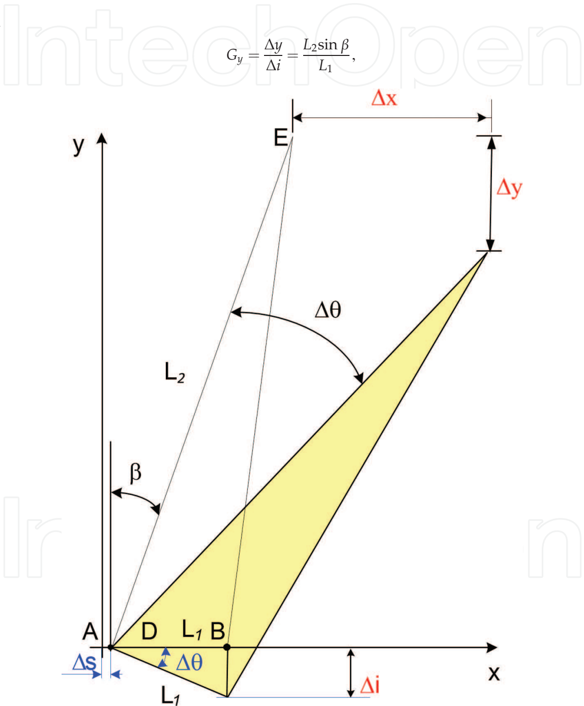
Figure 4. Kinematic motion relation of PLM in Figure 3 .
