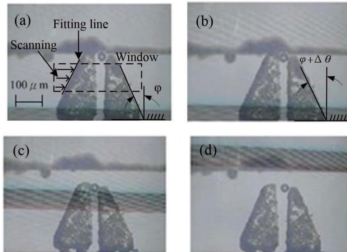
Figure 13. A microgripper is to approach (a), grasp (b), transport (c), and release (d) a 30 \mu m particle. The RSEF algorithm for measuring rotational angle is illustrated in (a) and (b).
