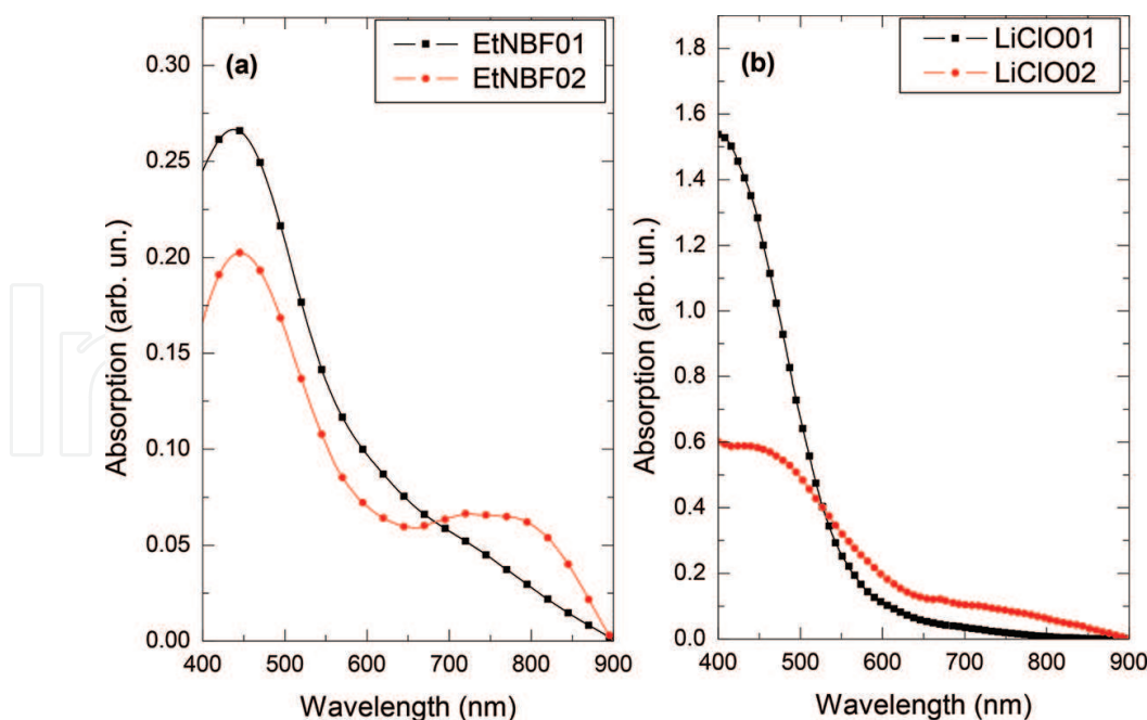
Figure 2. UV-Vis spectra for P3DDT films with one and two electropolymerization cycles: (a) EtNBF01 and EtNBF02 films and (b) LiClO01 and LiClO02 films.
