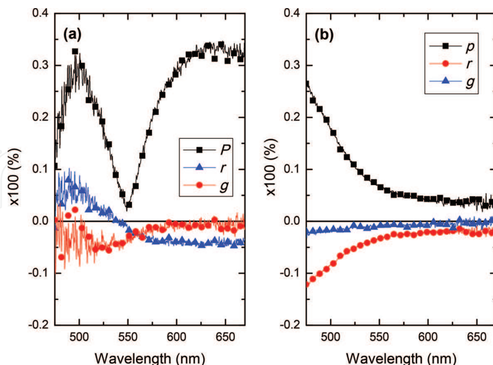
Figure 7. Polarization degree P , anisotropy factor r and dissymmetry factor g obtained from the Stokes parameters for the (a) EtNBF10 film and (b) LiClO4 film.
