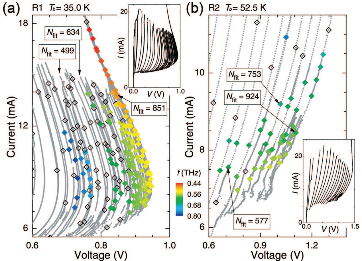
Figure 6. Emission at the color-coded frequencies was observed at the filled diamonds for R1 (a) and for R2 (b). No radiation was detected at the open diamonds. Arrows indicate the numbers of resistive junctions N_{\text{fit}} obtained from fits to the AC Josephson relation. The two insets show the full IVCs for each sample.
