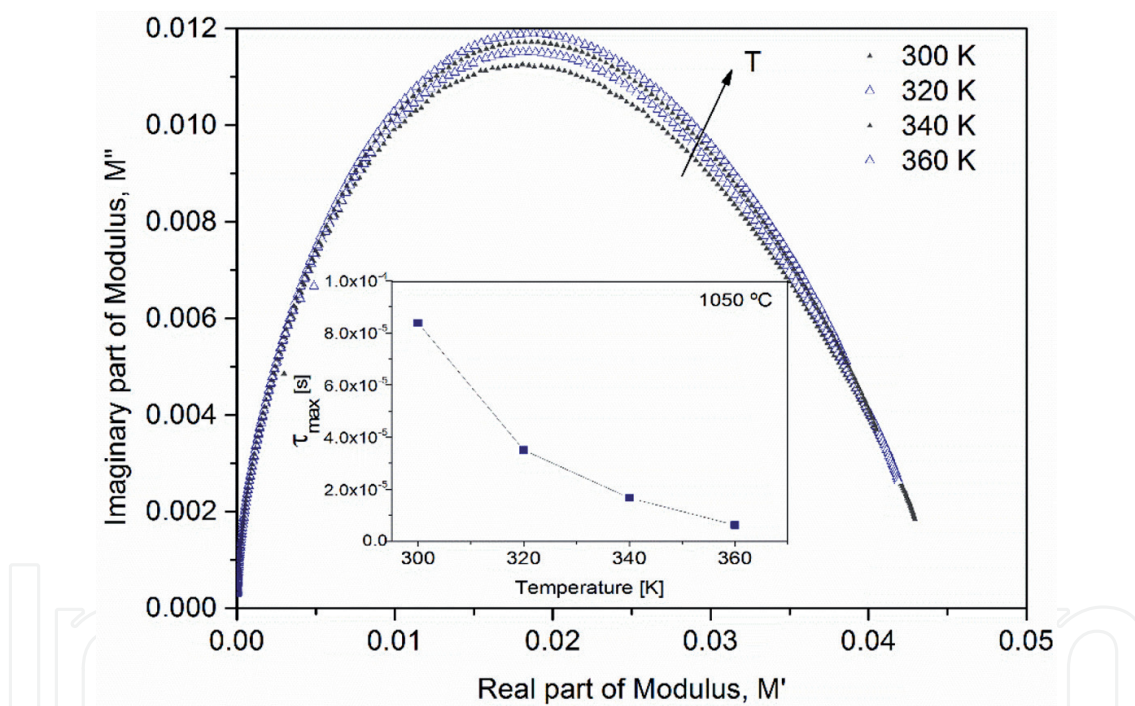
Figure 11. Nyquist plot for the sample treated at 1050°C for a range of temperatures between 300 and 360 K. Adapted from Ref. [14].
