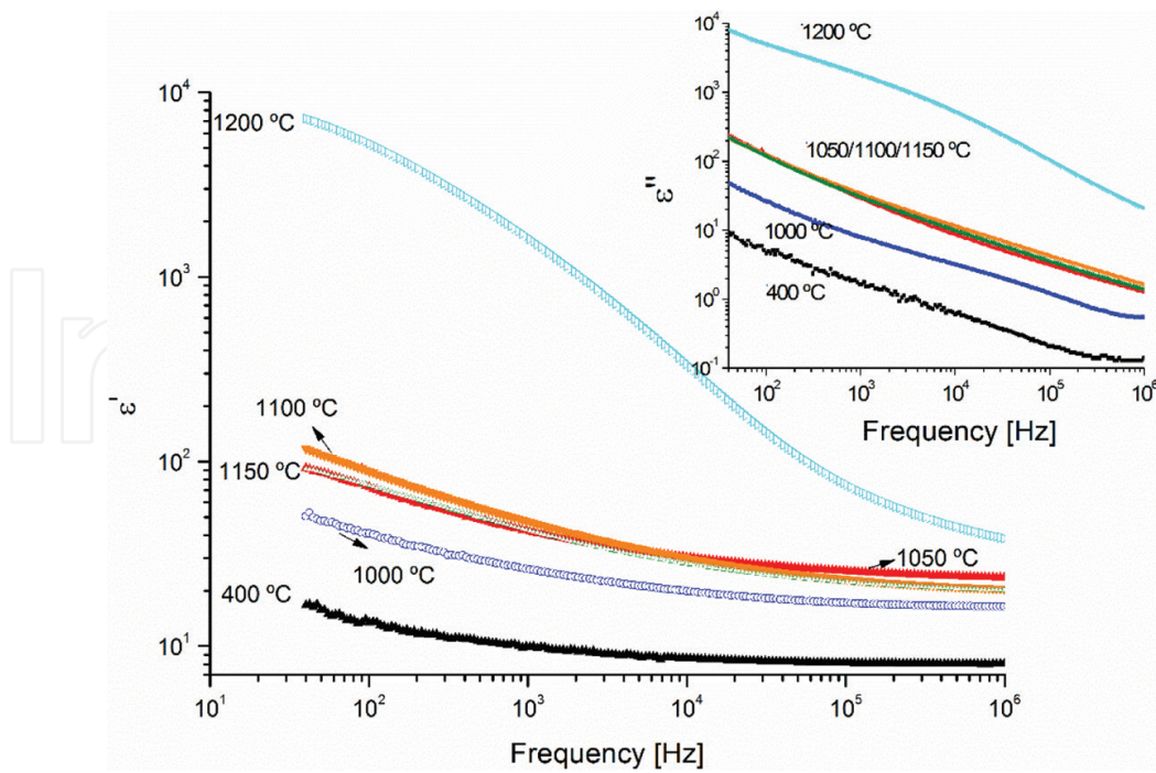
Figure 8. Frequency dependence of the complex permittivity, at T = 300 K [14].
