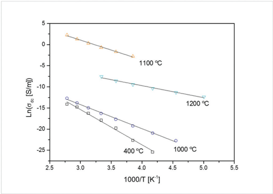
Figure 6. Log ( \sigma_{dc} ) versus 1000/T .
