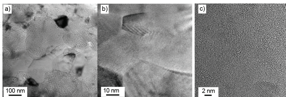
Figure 8. The structure of the aluminium alloy AlMg1SiCu composite material with reinforcement of the 15% halloysite nanotubes: (a) after mechanical alloying (STEM mode using the energy-filtered TEM microscopy technique), (b) and (c) with the occurrence of nanometric grains even 5–10 nm in the matrix (HRTEM).
