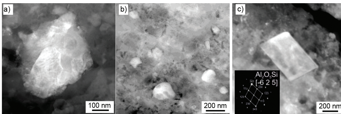
Figure 7. The structure of the aluminium alloy AlMg1SiCu composite material with reinforcement of the 15% halloysite nanotubes with the primary intermetallic phases: (a) \text{AlFe}_3 , (b) \text{Al}_4(\text{Fe, Cr, Mn})\text{Si}_{0.74} (c) \text{Al}_2\text{O}_5\text{Si} (TEM).
