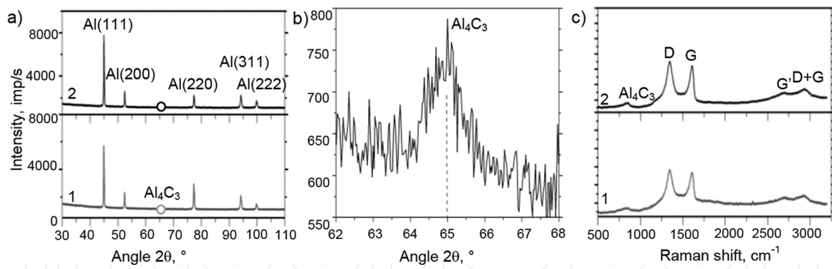
Figure 5. (a) X-ray diffraction pattern of nanocomposite material with volume fraction of 2% (1) and 5% (2) of MWCNTs for 10 h, (b) magnification of the peak of \text{Al}_4\text{C}_3 phase, (c) Raman spectrum of nanocomposite material with volume fraction of 2% (1) and 5% (2) of MWCNTs milled for 10 h.
