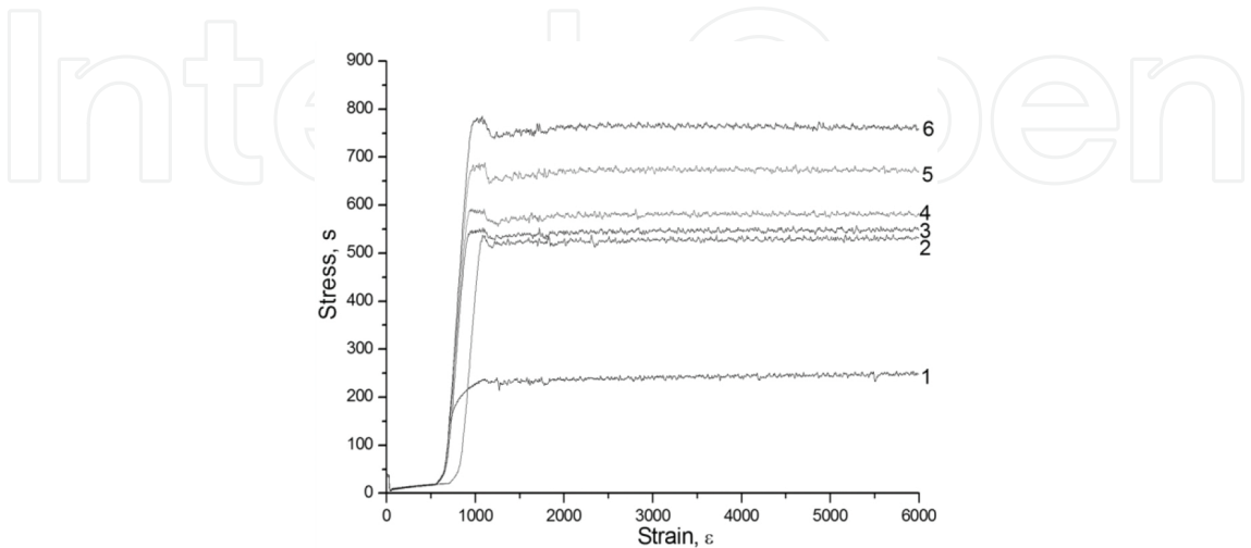
Figure 11. Compression test curves of the aluminium alloy EN AW-AlMg1SiCu composite materials with reinforcement of the different concentrations of carbon nanotubes: 1—AlMg1SiCu, 2—AlMg1SiCu/0%MWCNTs, 3—AlMg1SiCu/0.5%MWCNTs, 4—AlMg1SiCu/2%MWCNTs, 5—AlMg1SiCu/3.5%MWCNTs, 6—AlMg1SiCu/5%MWCNTs.
