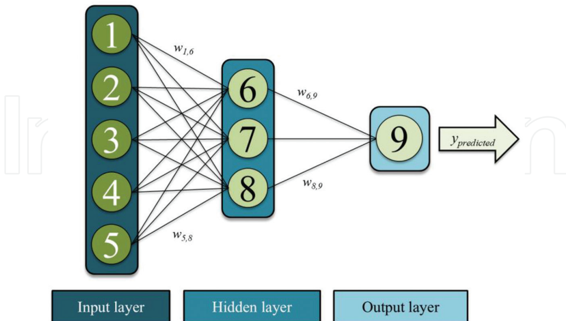
Figure 3. Example of neural model topology 5-3-1 with five neurons in the input layer, three neurons in intermediate layers and one neuron in the output layer.
