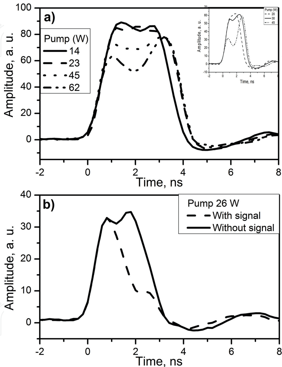
Figure 10. Pump pulses at the output of the FP filter when the SMF-28 fiber was used as the Fiber 1; (a) fiber length is equal to 300 m and the inset 600 m; (b) fiber length is equal to 1 km.
