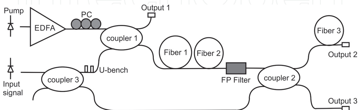
Figure 8. Experimental setup of Raman circuit.
