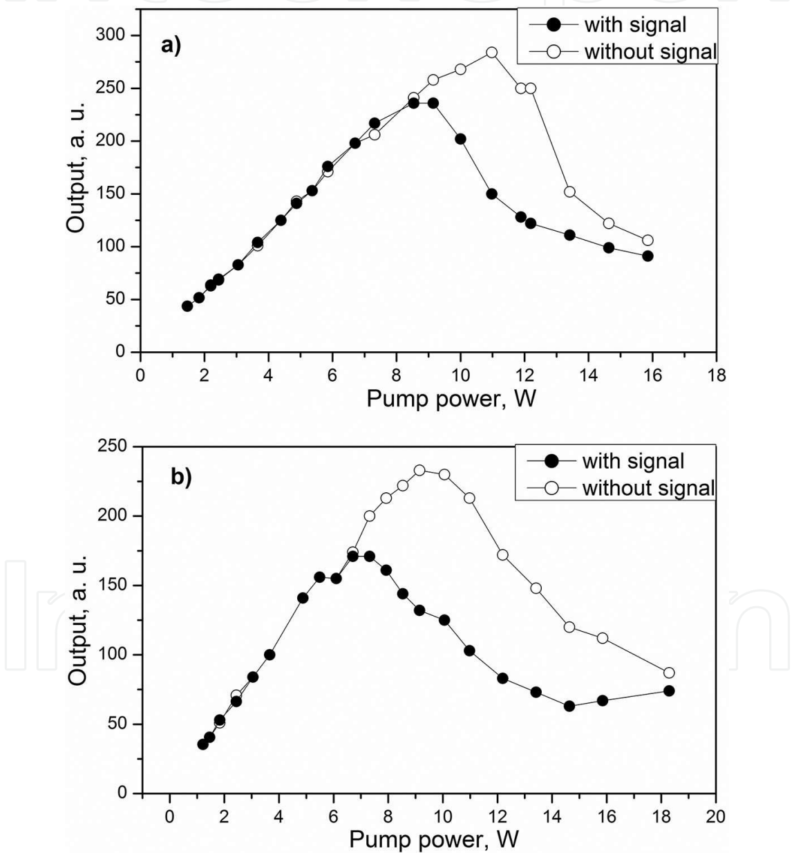
Figure 13. Saturation of peak power pump for variety of pump powers for two configurations: (a) 350 m SMF-LS fiber + 350 m SMF-28 fiber and (b) 350 m SMF-LS + 600 m SMF-28.
