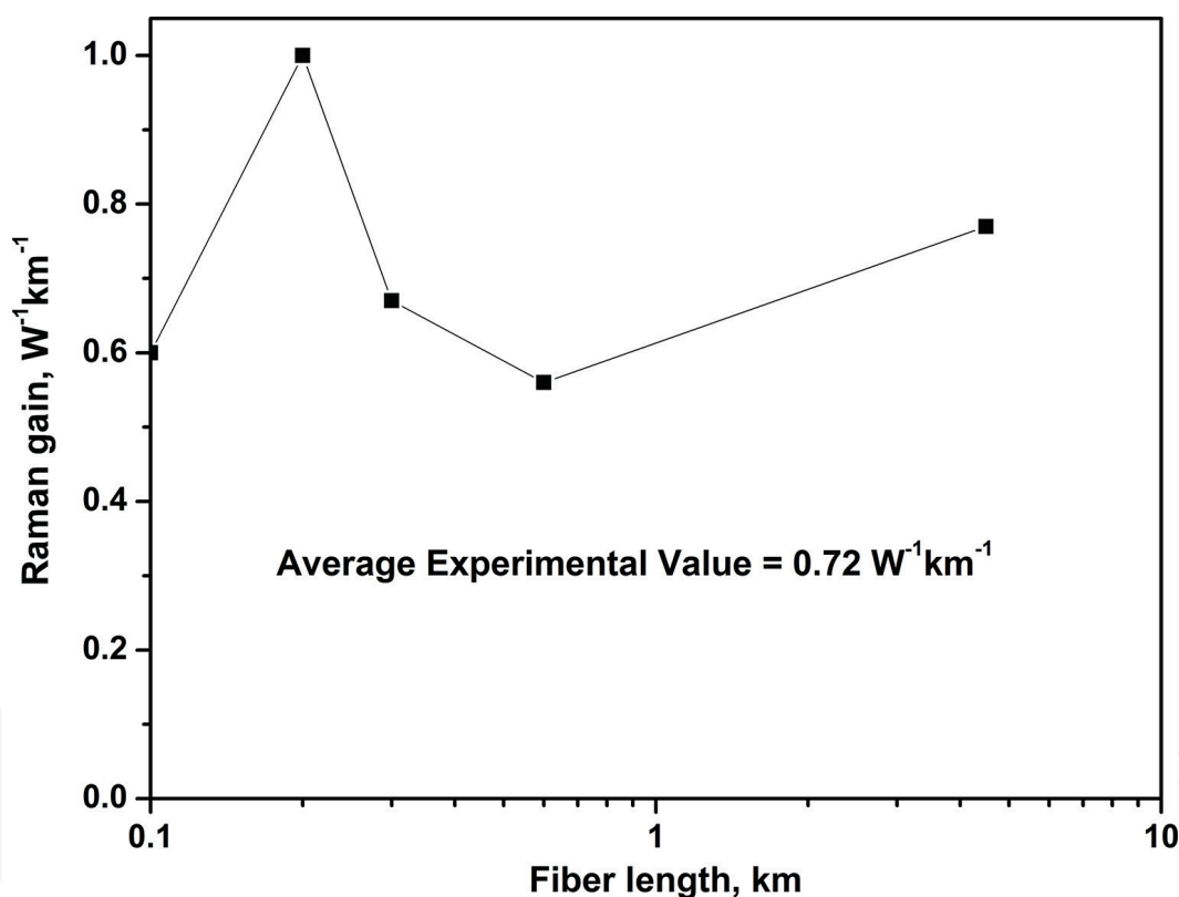
Figure 9. Raman gain.
