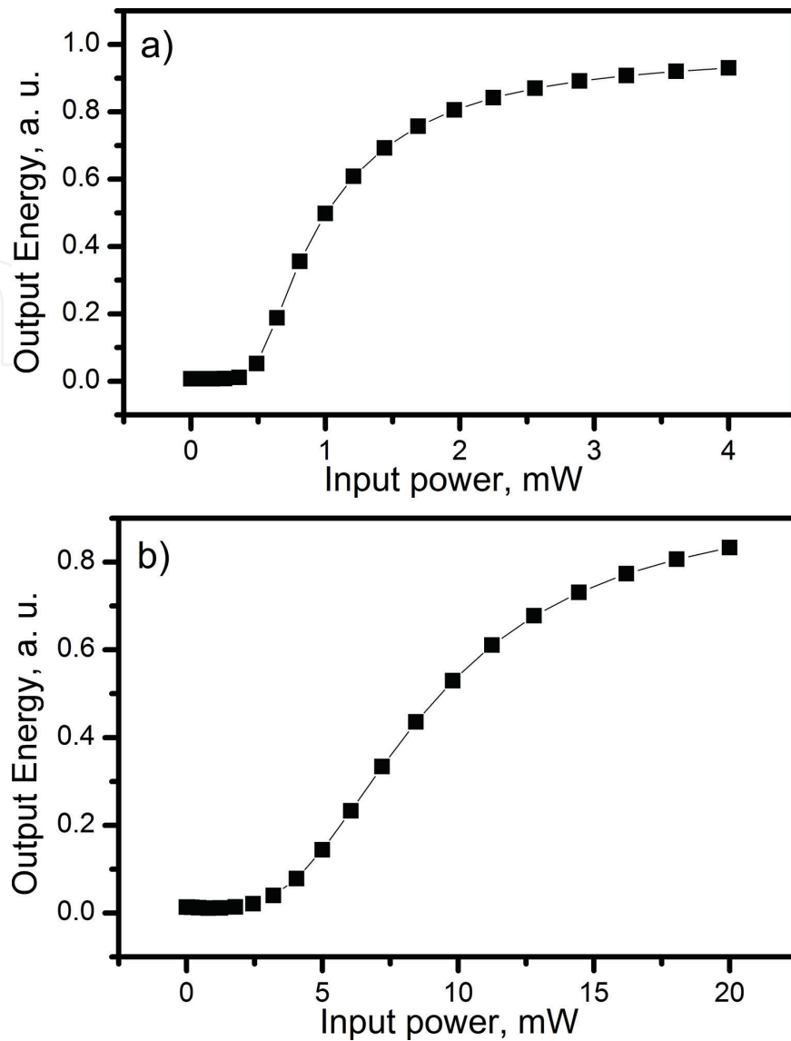
Figure 5. Dependencies of the output Stokes energy on the input power for two circuits connected in series: (a) attenuation is 10 times and (b) attenuation is 3 times.
