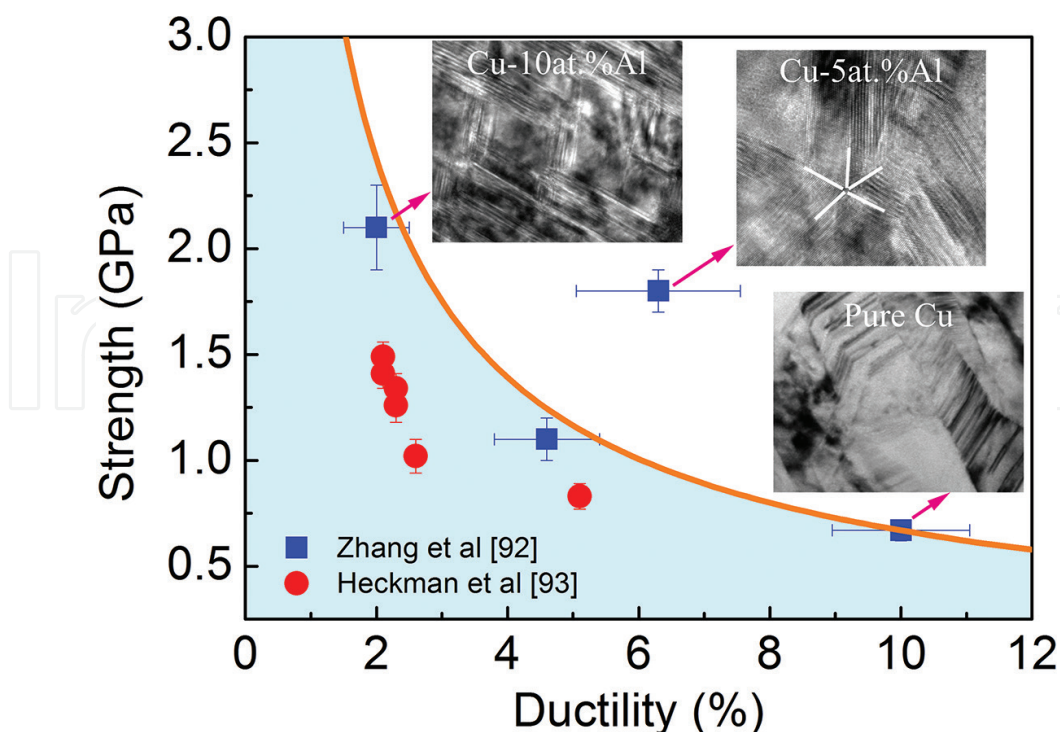
Figure 13. The strength-ductility tradeoff in Cu-Al alloyed thin films from literatures [92, 93]. Insets are the corresponding internal feature of Cu-Al films prepared by Zhang et al. [92].
