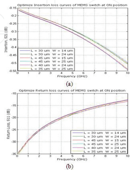
Figure 5. Optimized results at on-position of switch: (a) insertion and (b) return loss.
