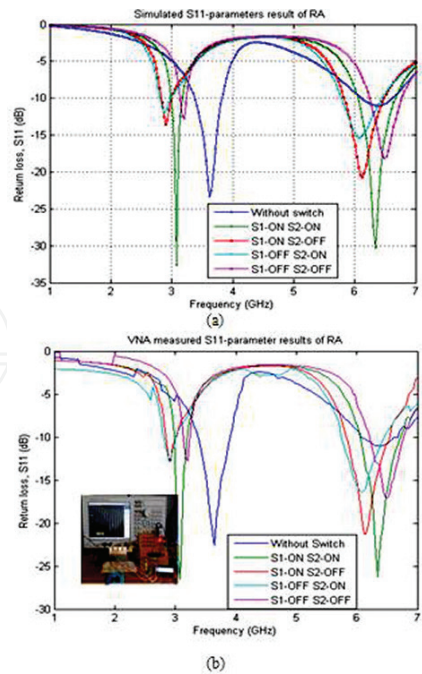
Figure 11. Comparison of simulated and measured RL of proposed RA.
