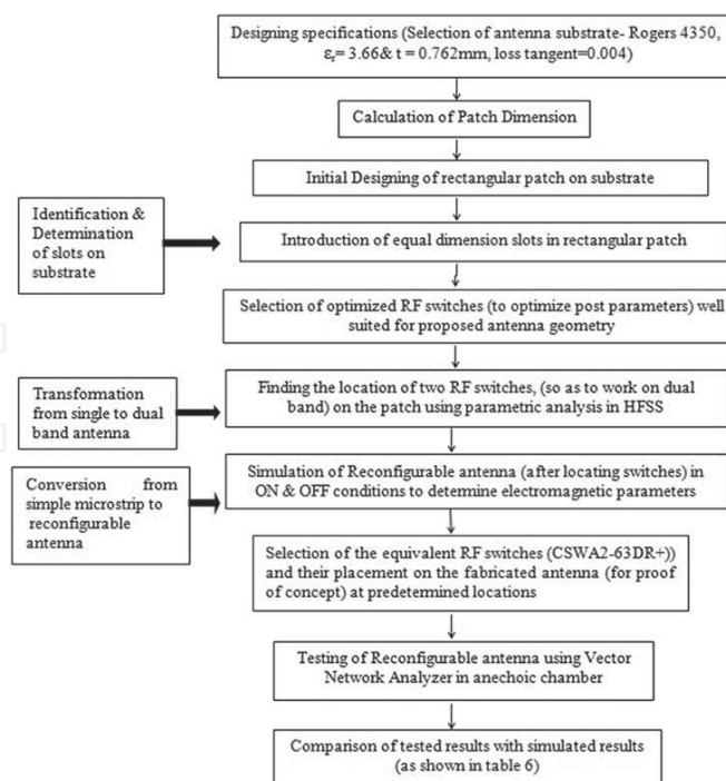
Figure 9. Flow diagram of designing approach of reconfigurable antenna.
