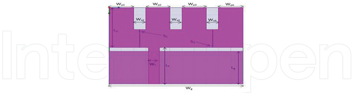
Figure 8. Dual band slot antenna with two metal-contact MEMS switches.
